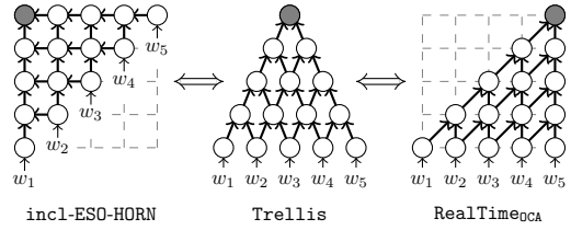
Figure 7. The bijection between incl-ESO-HORN and Trellis \square
