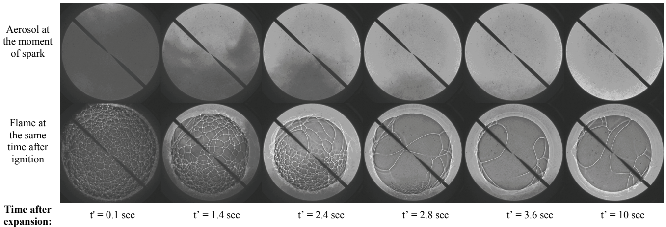
Fig. 3. Flame structures of ethanol-air mixtures at 60 °C, 4 bars and \text{Ø}=1.56 . All pictures are taken at 1.1ms after the flame ignition.
