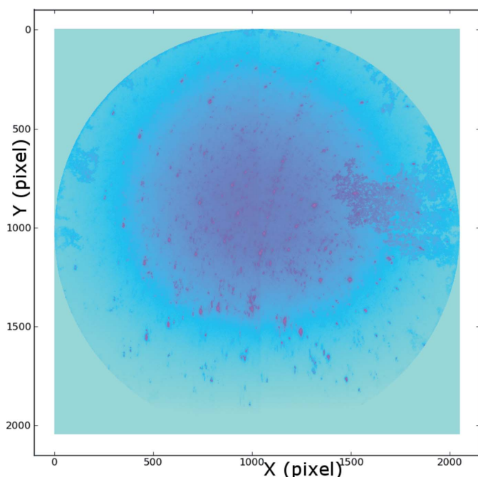
Figure 7 μLaue diffraction pattern of the sample, showing peaks from numerous ZrO 2 crystals. The splitting of a number of diffraction spots is due to the contribution of many different small crystals having slightly different orientations (within less than 0.5° of one another). A close-up is shown in Fig. 9.
