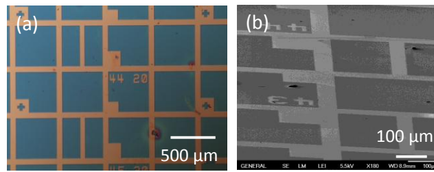
Figure 9 : (a) Optical and (b) SEM images of the patterns after lithography at 248 nm (10800 mJ.cm -2 ) and development in deionized water for 1 min. Patterns of the mask are non-exposed squares of 440 μm x 440 μm spaced of 60 μm exposed lines.
