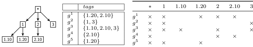
Fig. 2: A tree of tags (left), a set of tagged items (middle) and its flat representation (right)
