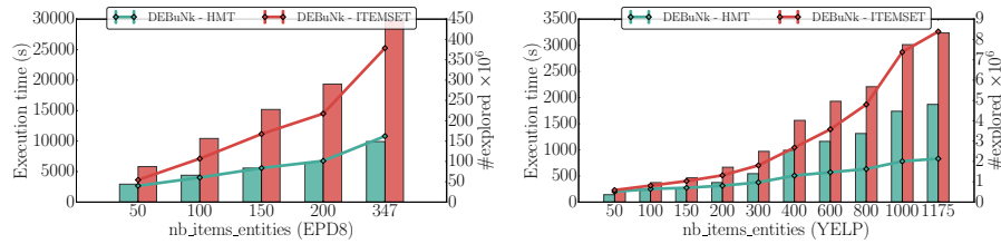
Fig. 13: Efficiency of HMT against itemsets closed descriptions enumeration according to the number of items/tags constituting the hierarchy for the two datasets EPD8 (left) and Yelp (right). For both datasets we only consider the HMT attribute for entities |\mathcal{A}_E| = 1 . The used parameters for EPD8 are: |\mathcal{A}_I| = 6 , \sigma_E = 1 , \sigma_I = 10 , \sigma_\varphi = 0.5 and \varphi_{dissent} . The used parameters for Yelp are: |\mathcal{A}_I| = 3 , \sigma_E = 5 , \sigma_I = 1 , \sigma_\varphi = 0.5 and \varphi_{dissent} .
