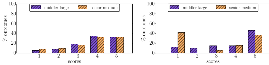
Fig. 21: Pattern 2 Illustration - distribution of ratings of individuals constituting the group of Yelp user registered in between 2010-2015 having a large friend network versus distribution of ratings of individuals constituting the group of Yelp users registered before 2010 having a medium friend network. Left figure corresponds to the usual distribution observed over all Yelp places. Right figure corresponds to the contextual distribution observed over Nevada's Internal Medicines Places.
