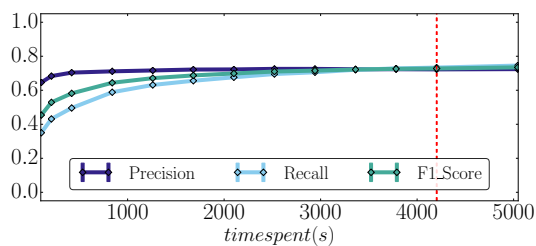
Fig. 27: Efficiency of Quick- DEBuNk compared to DEBuNk over Openmedic. We consider the full dataset (i.e. all attributes and all records), the parameters used for Openmedic are \sigma_E = 5 , \sigma_I = 1 , \sigma_\varphi = 5 and \varphi_{ratio} .
