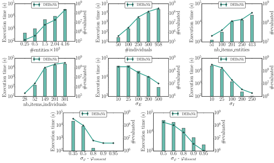
Fig. 14: Effectiveness of DEBuNk over EPD8 according to the sizes of E , I , \mathcal{D}_E , \mathcal{D}_I , the supports and quality measures thresholds. Considering by default |G_E| = 4161 , |G_I| = 958 , |Outcomes| = 750k , |\mathcal{A}_E| = 3 , |\mathcal{A}_I| = 6 . \sigma_E = 40 , \sigma_I = 10 , \sigma_\varphi = 0.5 and \varphi_{dissent} .
