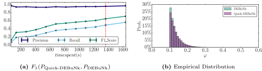
Fig. 19: Efficiency of Quick-DEBuNk compared to DEBuNk over Yelp. Parameters used are \sigma_E = 15 , \sigma_I = 1 , \sigma_\varphi = 0.1 and \varphi_{dissent} . The red line in each figure correspond to the required time by DEBuNk to perform an exhaustive search.
