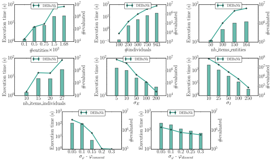
Fig. 15: Effectiveness of DEBuNk over Movielens Dataset according to the sizes of E , I , \mathcal{D}_E , \mathcal{D}_I , the supports and quality measures thresholds. Considering by default the full dataset. \sigma_E = 8 , \sigma_I = 50 , \sigma_\varphi = 0.2 and the quality \varphi_{dissent}
