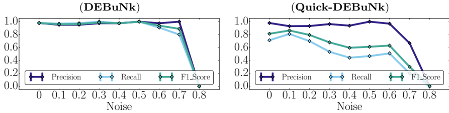
Fig. 9: Efficiency of DEBuNk ( \sigma_E = 7 , \sigma_I = 7 , \sigma_\varphi = 0.5 and \varphi_{dissent} ) and Quick-DEBuNk ( \sigma_E = 7 , \sigma_I = 7 , \sigma_\varphi = 0.5 , timebudget = 3\text{ mn} and \varphi_{dissent} ) performed over 21 behavioral artificial data generated with the following default parameters ( |G_E| = 2000 , |G_I| = 500 , |\mathcal{A}_E| = |\mathcal{A}_I| = 3 , size\_dom\_entities\_attributes = size\_dom\_individuals\_attributes = 4 , nb\_hidden\_patterns = 5 , context\_support\_size = 10 , group\_support\_size = 10 ).
