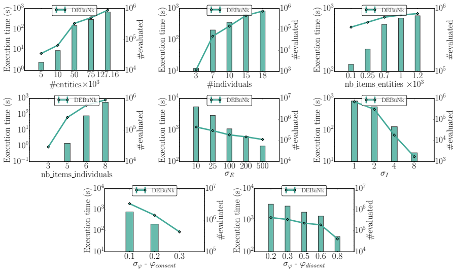
Fig. 16: Effectiveness of DEBuNk over Yelp Dataset according to the size of E , I , \mathcal{D}_E , \mathcal{D}_I , the supports and the quality measures thresholds. Considering by default the full dataset. \sigma_E = 50 , \sigma_I = 1 , \sigma_\varphi = 0.5 and the quality \varphi_{dissent}
