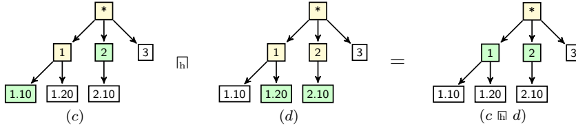
Fig. 3: Illustration of the infimum operator \sqcap
