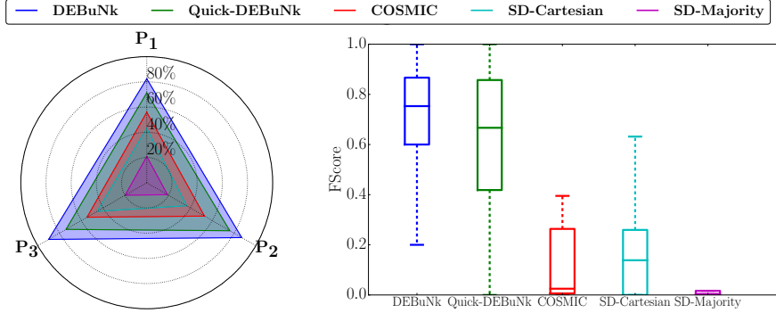
(a) Average similarity between the planted patterns and their representatives returned by each method.
