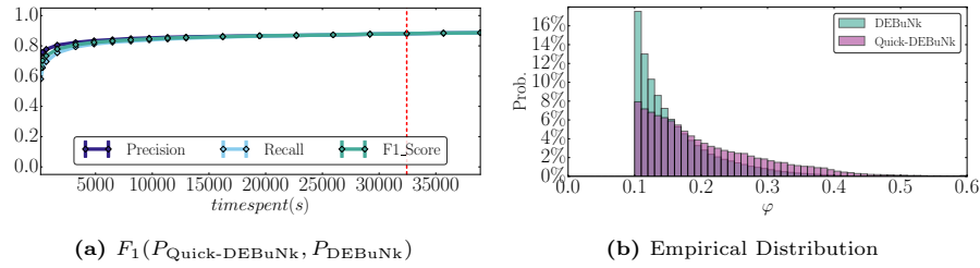
Fig. 17: Efficiency of Quick-DEBuNk compared to DEBuNk over EPD8. Parameters used are \sigma_E = 40 , \sigma_I = 10 , \sigma_\varphi = 0.5 and \varphi_{dissent} . The red line in each figure correspond to the required time by DEBuNk to perform an exhaustive search.
