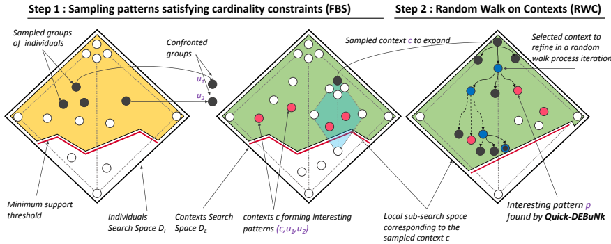
Fig. 4: Quick-DEBuNk approach in a nutshell
