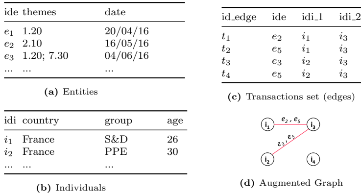
Fig. 5: Example of input data format for Cosmic after transforming the behavioral dataset given in Table 1 to an augmented graph and its corresponding transactions set according to the observed discords.
