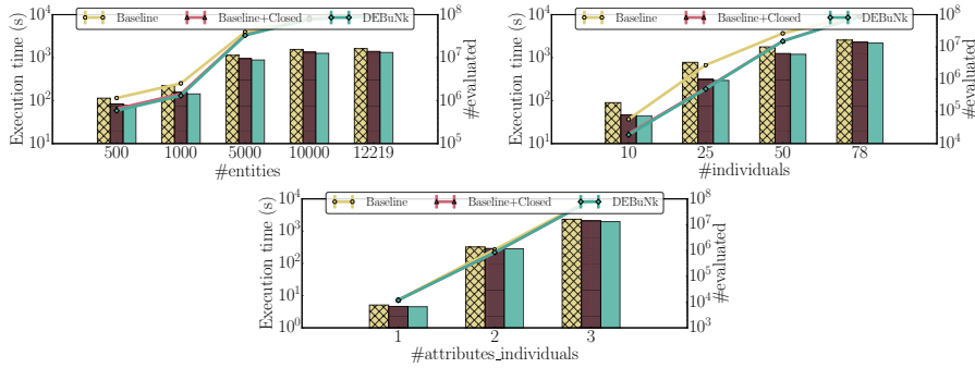
Fig. 25: Effectiveness of DEBuNk over Openmedic Dataset considering |G_E| = 12219 , |G_I| = 78 , |Outcomes| = 500k , |\mathcal{A}_E| = 1 , |\mathcal{A}_I| = 3 , \sigma_E = 5 , \sigma_I = 1 , \sigma_\varphi = 5 and the quality measure \varphi_{ratio}
