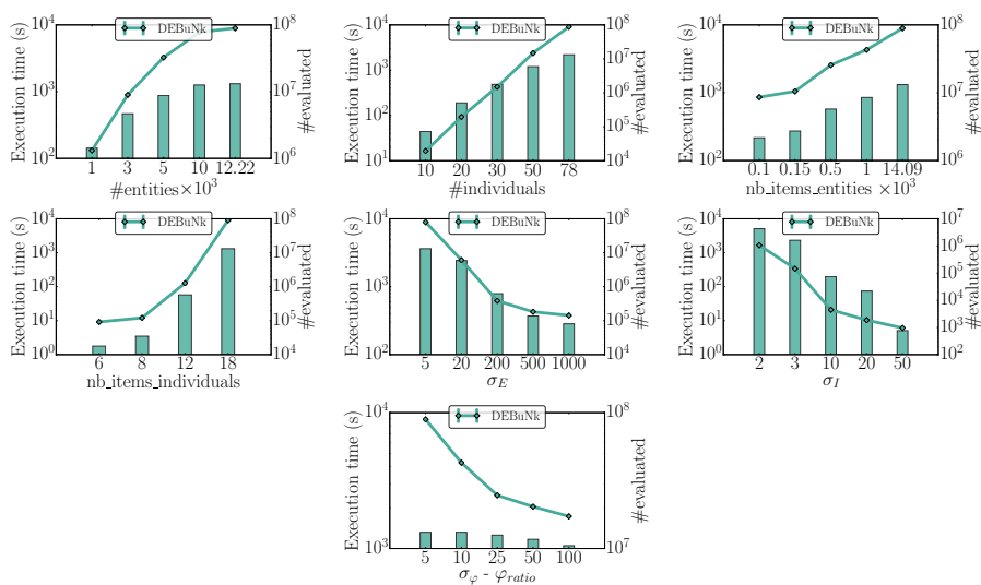
Fig. 26: Effectiveness of DEBuNk over Openmedic Dataset according to the sizes of E , I , \mathcal{D}_E , \mathcal{D}_I , the supports and quality measures thresholds. Considering by default the full dataset. \sigma_E = 5 , \sigma_I = 1 , \sigma_\varphi = 5 and the quality \varphi_{ratio}
