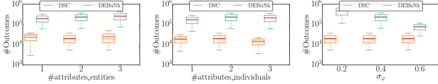
Fig. 8: Comparison between DEBuNk and DSC (top-k) for the task of discovering k -sized pattern set. Experiments consider the full EPD8 Dataset with the following default parameters: |\mathcal{A}_E| = 2 , |\mathcal{A}_I| = 2 , \sigma_\varphi = 0.4 , \sigma_E = 40 , \sigma_I = 10 and \varphi_{dissent} . Box plots correspond to the size of O[P^k] when varying k in [10, 50, 100] .
