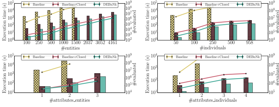
Fig. 10: Effectiveness of DEBuNk considering EPD8 Dataset with |G_E| = 2000 , |G_I| = 500 , |Outcomes| = 750k , |\mathcal{A}_E| = 3 , |\mathcal{A}_I| = 4 , \sigma_E = 40 , \sigma_I = 10 , \sigma_\varphi = 0.5 and \varphi_{dissent} . Lines correspond to the execution time and bars correspond to the number of evaluated patterns.
