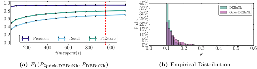
Fig. 18: Efficiency of Quick-DEBuNk compared to DEBuNk over MOVIELENS. Parameters used are \sigma_E = 5 , \sigma_I = 10 , \sigma_\varphi = 0.25 and \varphi_{dissent} . The red line in each figure correspond to the required time by DEBuNk to perform an exhaustive search.
