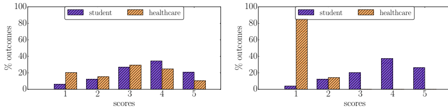
Fig. 20: Pattern 1 Illustration - distribution of ratings of individuals constituting the group of students versus distribution of ratings of individuals constituting the group of healthcare professionals. Left figure corresponds to the usual distribution observed over all movies. Right figure corresponds to the contextual distribution observed over the context highlighted by pattern 1
