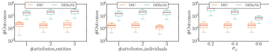
Fig. 8: Comparison between DEBuNk and DSC (top-k) for the task of discovering k -sized pattern set. Experiments consider the full EPD8 Dataset with the following default parameters: |\mathcal{A}_E| = 2 , |\mathcal{A}_I| = 2 , \sigma_\varphi = 0.4 , \sigma_E = 40 , \sigma_I = 10 and \varphi_{dissent} . Box plots correspond to the size of O[P^k] when varying k in [10, 50, 100] .
