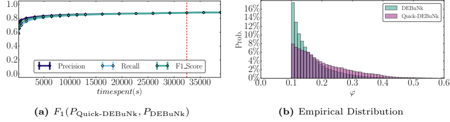
Fig. 17: Efficiency of Quick-DEBuNk compared to DEBuNk over EPD8. Parameters used are \sigma_E = 40 , \sigma_I = 10 , \sigma_\varphi = 0.5 and \varphi_{\text{dissent}} . The red line in each figure correspond to the required time by DEBuNk to perform an exhaustive search.
