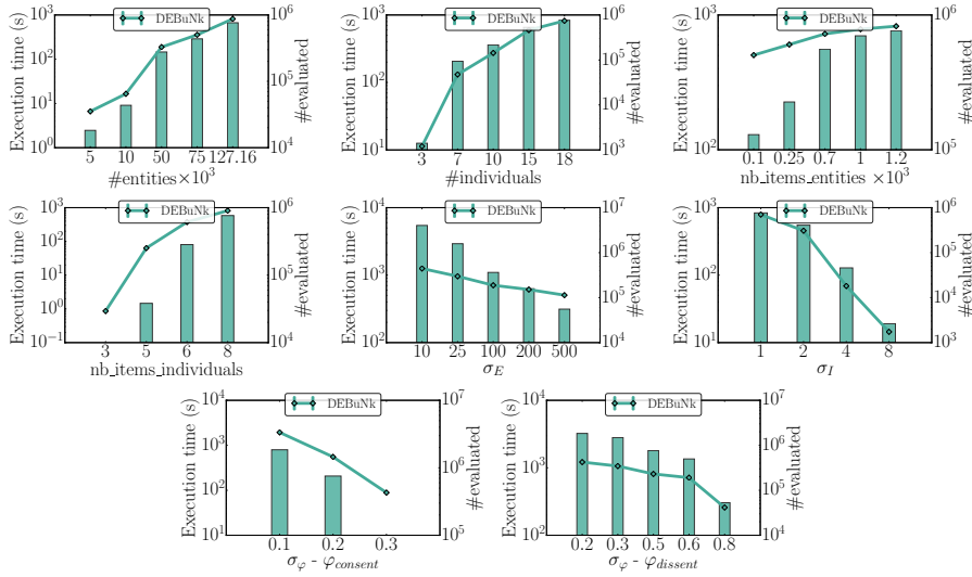
Fig. 16: Effectiveness of DEBuNk over Yelp Dataset according to the size of E , I , \mathcal{D}_E , \mathcal{D}_I , the supports and the quality measures and the quality thresholds. Considering by default the full dataset. \sigma_E = 50 , \sigma_I = 1 , \sigma_\varphi = 0.5 and the quality \varphi_{dissent}
