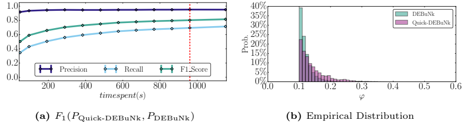
Fig. 18: Efficiency of Quick-DEBuNk compared to DEBuNk over MOVIELENS. Parameters used are \sigma_E = 5 , \sigma_I = 10 , \sigma_\varphi = 0.25 and \varphi_{\text{dissent}} . The red line in each figure correspond to the required time by DEBuNk to perform an exhaustive search.
