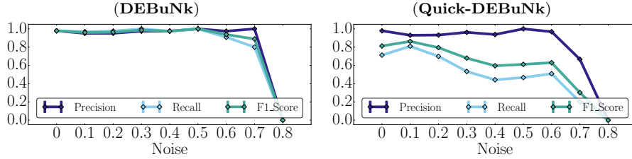
Fig. 9: Efficiency of DEBuNk ( \sigma_E = 7 , \sigma_I = 7 , \sigma_\varphi = 0.5 and \varphi_{dissent} ) and Quick-DEBuNk ( \sigma_E = 7 , \sigma_I = 7 , \sigma_\varphi = 0.5 , timebudget = 3\ mn and \varphi_{dissent} ) performed over 21 behavioral artificial data generated with the following default parameters ( |G_E| = 2000 , |G_I| = 500 , |\mathcal{A}_E| = |\mathcal{A}_I| = 3 , size\_dom\_entities\_attributes = size\_dom\_individuals\_attributes = 4 , nb\_hidden\_patterns = 5 , context\_support\_size = 10 , group\_support\_size = 10 ).
