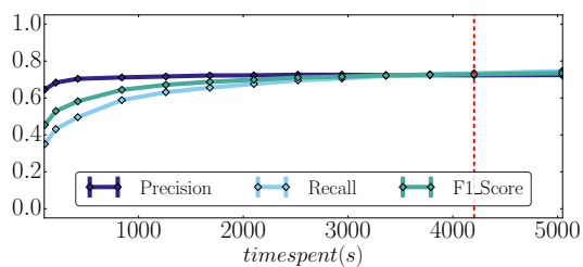
Fig. 27: Efficiency of Quick-DEBuNk compared to DEBuNk over Openmedic. We consider the full dataset (i.e. all attributes and all records), the parameters used for Openmedic are \sigma_E = 5 , \sigma_I = 1 , \sigma_\varphi = 5 and \varphi_{ratio} .
