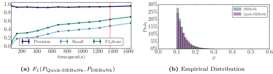
Fig. 19: Efficiency of Quick-DEBuNk compared to DEBuNk over Yelp. Parameters used are \sigma_E = 15 , \sigma_I = 1 , \sigma_\varphi = 0.1 and \varphi_{\text{dissent}} . The red line in each figure correspond to the required time by DEBuNk to perform an exhaustive search.
