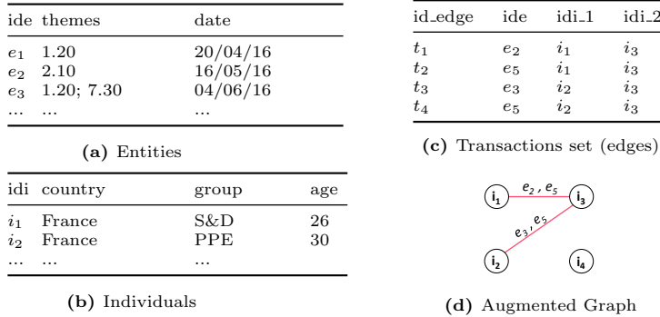
Fig. 5: Example of input data format for Cosmic after transforming the behavioral dataset given in Table 1 to an augmented graph and its corresponding transactions set according to the observed discords.
