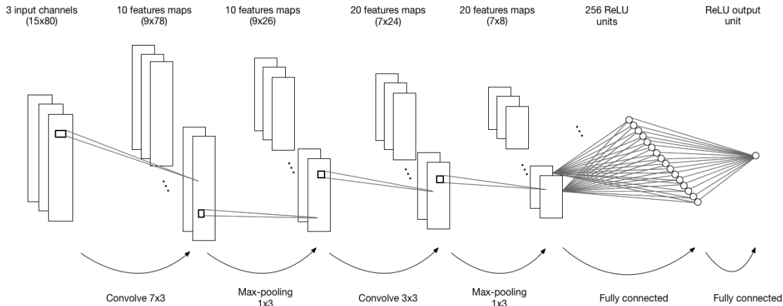
Figure 1: Convolutional neural network used for this work.
