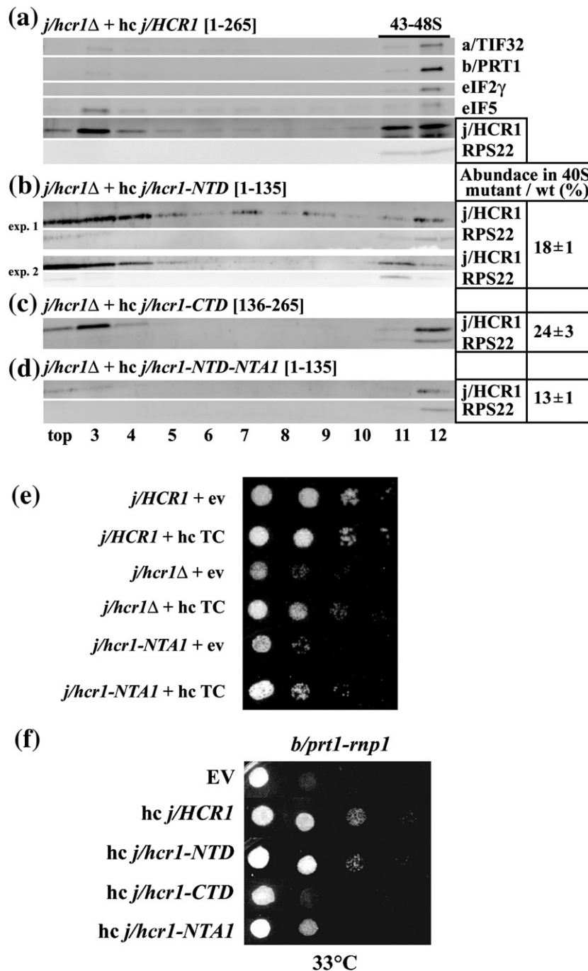
Fig. 2. Both the NTD and the CTD of j/HCR1 retain intrinsic 40S binding affinity. (a–d) Transformants of strain H428 ( j/hcr1Δ ) bearing YEp- j/HCR1 -DS, YEp- j/hcr1-NTD , YEp- j/hcr1-CTD , and YEp- j/hcr1-NTD-NTA1 , respectively, were grown in SD medium at 30 °C to an OD 600 of ~1.5 and cross-linked with 2% HCHO prior to harvesting. WCEs were prepared and subsequently separated on a 7.5–30% sucrose gradient by centrifugation at 41,000 rpm for 5 h. The 40S fractions were pooled, resolved on a second gradient, and subjected to Western blot analysis. The first two fractions were combined (top). Proportions of the 40S-bound j/HCR1 proteins relative to the amount of 40S subunits were calculated, using NIH ImageJ, from two independent experiments. The resulting values obtained with the wt strain were set to 100%, and those obtained with mutant strains were expressed as percentages of wt (SD given). (e–f) Genetic evidence that j/HCR1 with intact NTA (or only its NTD) stimulates 40S binding by eIF3. (e) Overexpression of TC partially suppresses the Slg - phenotype of j/hcr1Δ and j/hcr1-NTA1 mutants. H416 ( j/HCR1 ; rows 1 and 2), H428 ( j/hcr1Δ YEplac181; rows 3 and 4), and SY73 ( j/hcr1Δ YEp- j/hcr1-NTA1 ; rows 5 and 6) were transformed with either the empty vector (rows 1, 3, and 5) or the TC-overexpressing vector (rows 2, 4, and 6), and the resulting transformants were spotted in four serial 10-fold dilutions on SD medium and incubated at 30 °C for 2 days. (f) j/HCR1 with intact NTA (or only its NTD) partially suppresses the temperature-sensitive (Ts - ) phenotype of b/prt1-rnp1 . Transformants of the strain H3674 ( b/prt1-rnp1 ) 12 bearing the empty vector, YEp- j/HCR1 -DS, YEp- j/hcr1-NTD , YEp- j/hcr1-CTD , and YEp- j/hcr1-NTA1 , respectively, were spotted in four serial 10-fold dilutions on SD medium and incubated at 33 °C for 3 days.
