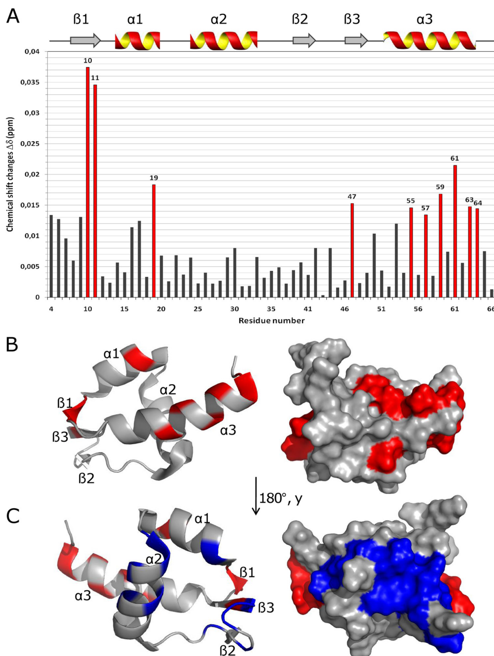
FIGURE 5. Mapping the binding site of DnaJ in the TorI structure by heteronuclear NMR. A , plot of the weighted average chemical shift variations of ^{15}\text{N} -TorI backbone upon binding of DnaJ. Secondary structures of TorI are shown above the plot. The red bars correspond to residues showing the largest chemical shift variations. B , chemical shift mapping onto ribbon (right) and surface (left) representations of TorI. Residues undergoing the largest chemical shift changes upon DnaJ binding are colored in red. C , ribbon (right) and surface (left) representations of the data presented in B , after 180° rotation according to the y axis, with the residues involved in DNA binding colored blue.
