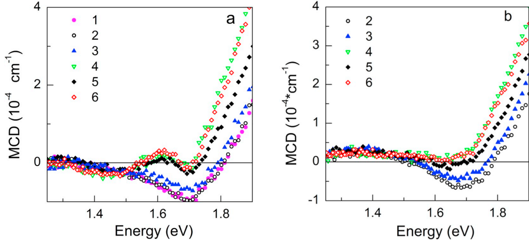
Fig. 7. MCD spectra for samples 1 to 6 at 295 (a) and 90 K (b) measured in the magnetizing field of 0.35 T. The curve numbers correspond to the sample numbers.
