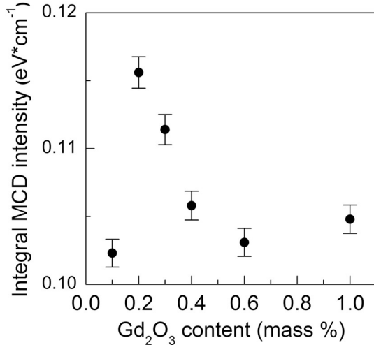
Fig. 6. Integral MCD intensity vs. \text{Gd}_2\text{O}_3 contents, calculated as the area under the spectral curves in the range of 2.0 to 3.0 eV. The error bars show the accuracy of measurements.
