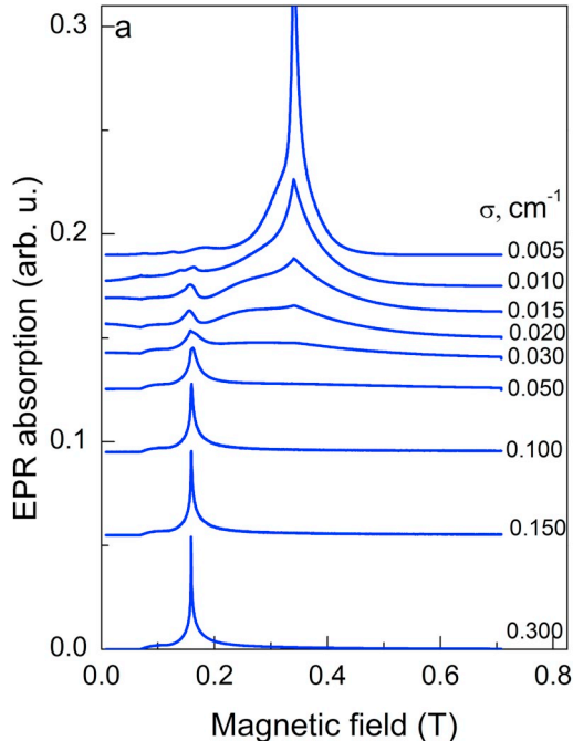
Fig. 12. Computer-generated X band EPR absorption spectra of \text{Fe}^{3+} (a) and \text{Gd}^{3+} ions (b) for D_0 = 0 and E_0 = 0 , and different \sigma -values shown alongside the curves.
