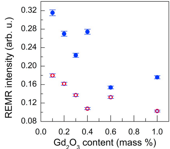
Fig. 15. REMR absorption intensities at different \text{Gd}_2\text{O}_3 contents at 120 K (full circles, blue online) and 300 K (empty circles, red online). (For interpretation of the references to colour in this figure legend, the reader is referred to the web version of this article.)
