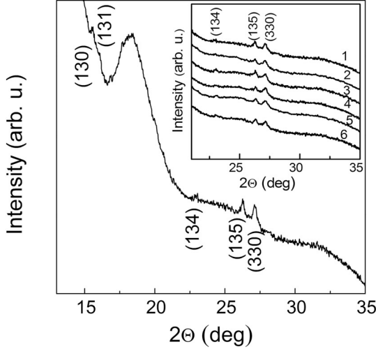
Fig. 3. XRD patterns for sample 1 measured at the wavelength of 0.696585 Å. The inset shows the XRD patterns for all samples measured at the same wavelength in a narrower angular range; the curve numbers are the sample numbers. The indices of some \epsilon -Fe 2 O 3 reflections are shown.
