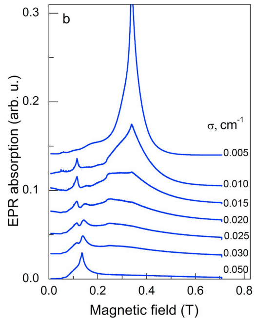
Fig. 12. Computer-generated X band EPR absorption spectra of \text{Fe}^{3+} (a) and \text{Gd}^{3+} ions (b) for D_0 = 0 and E_0 = 0 , and different \sigma -values shown alongside the curves.
