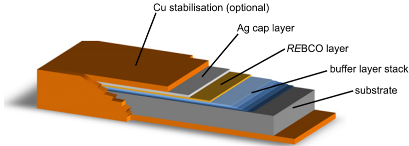
Fig. 1. Schematic layout of REBCO tapes. The layers are not up to scale (courtesy C. Barth, University of Geneva).
