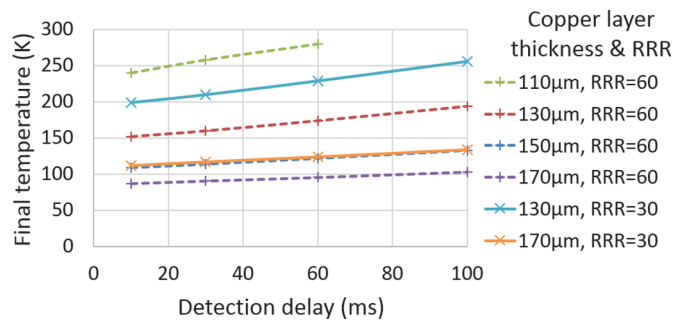
Fig. 11. Maximal hotspot temperature as a function of detection delay for different copper thicknesses and different RRR.
