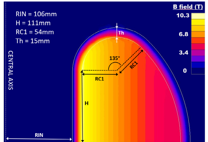
Fig. 9. View of a half D-shape section. The magnetic field is 0 outside the torus, B is decreasing inversely proportional with the distance to torus central axis.
