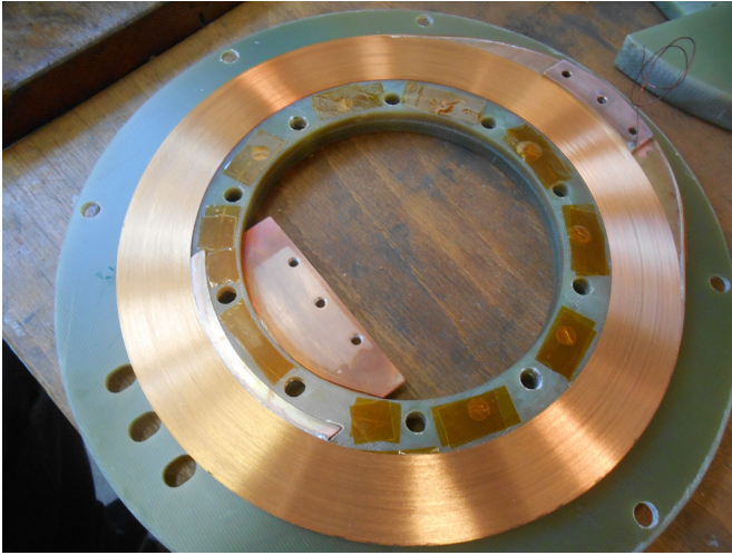
Fig. 7. View of a prototype pancake. The mandrel, the internal contact, the winding, the external contact and a flange are visible.
