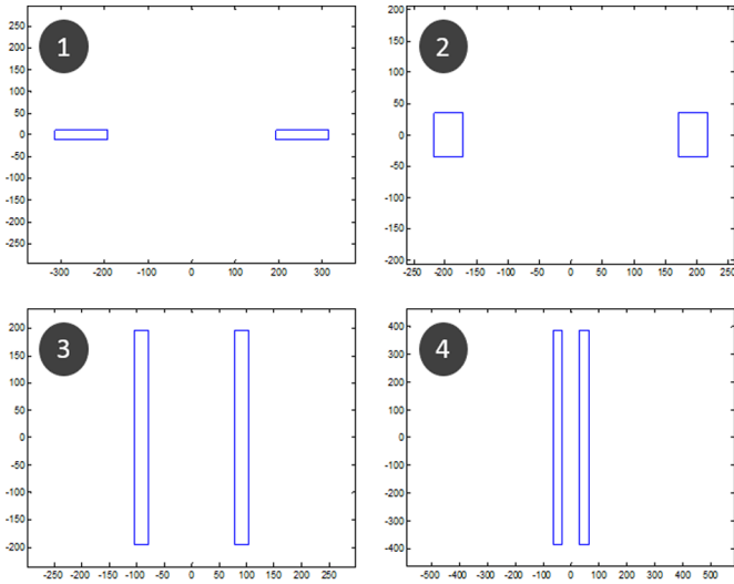
Fig. 5. Cross section view of solenoids 1, 2, 3 and 4 identified in Figure 6. Topology evolution is visible. Axes are graduated in mm.
