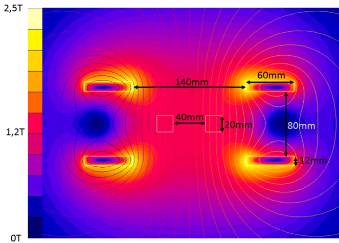
Fig. 14. Cross section view of induction field when the coil is charged, just before launching. The field between the rails is then 1.2 T. At the beginning of the launch, the field rises until 1.4 T (additional field generated by current the rails).
