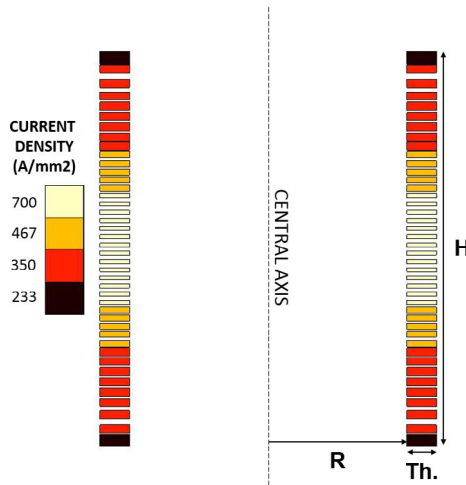
Fig. 8. Cross section view of the solenoid. As the tapes are wider, the current density is lower at solenoid extremities. R = 135 mm, TH = 29 mm, H = 384 mm.
