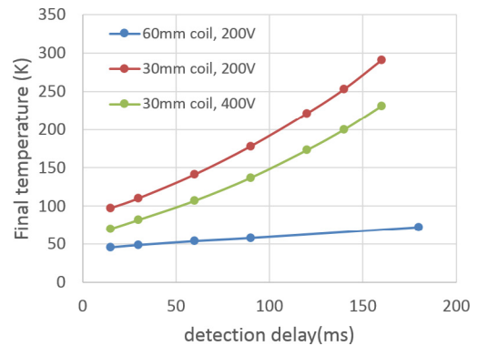
Fig. 15. Maximal hotspot temperature as a function of detection delay, in two different configurations (total thickness of the winding = 30 or 60 mm) and different discharge voltage. RRR = 15.
