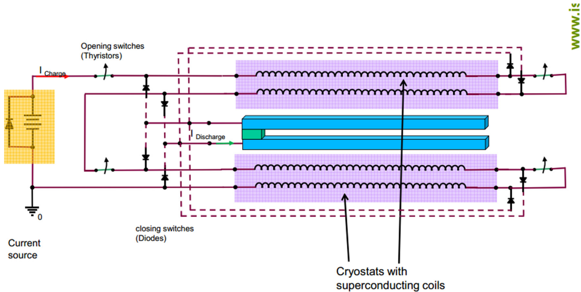
Fig. 13. Principle diagram of the launcher electrical circuit (courtesy V. Brommer, ISL).
