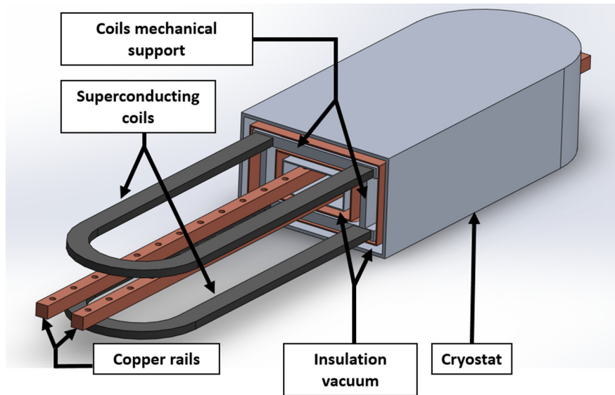
Fig. 12. CAO plan of the S3EL launcher (courtesy R. Pasquet, SigmaPhi).
