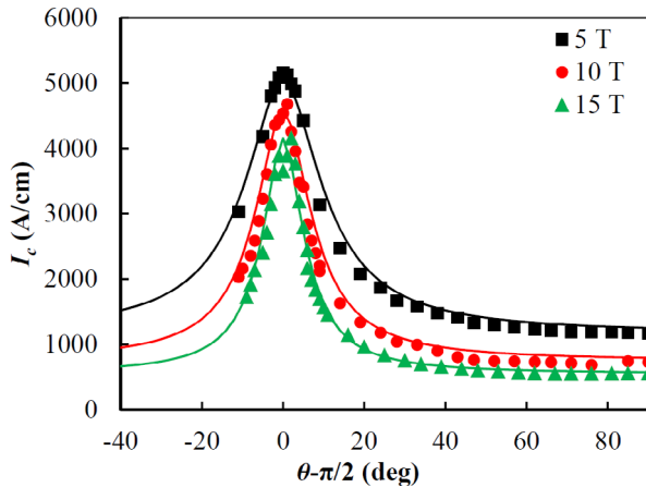
Fig. 3. Critical current of a Fujikura REBCO tape at 4.2 K with value of B field and its deviation to tape's surface. Data from Tohoku University [17], fit by Fleiter [18].
