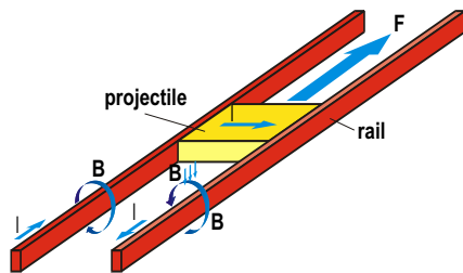
Fig. 2. Principle diagram of an electromagnetic launcher (railgun) and picture of the PEGASUS launcher (10 MJ).
