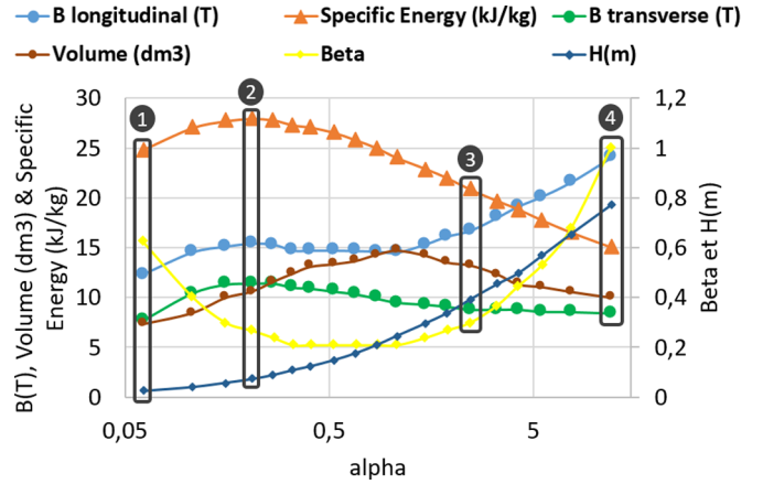
Fig. 6. Set of topological solutions respecting E=1 MJ, \sigma=500 MPa, and J=600 A/mm 2 for different values of aspect ratio \alpha . Solutions at the left are corresponding to flat solenoids, and solutions on the right are very long solenoids. B longitudinal is the maximum B field in mid-plan of the coil and B transverse is the maximum radial B field (at the top and middle of coil's section). H is the height.
