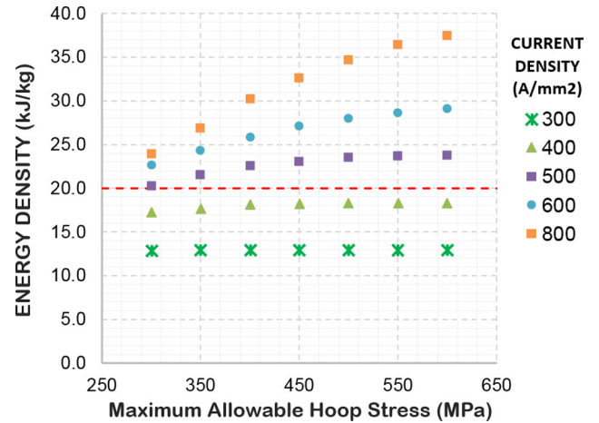
Fig. 4. Maximum possible specific energy as a function of maximum allowable hoop stress and for several current densities ( \rho = 8900 \text{ kg/m}^3 , E = 1 \text{ MJ} ).
