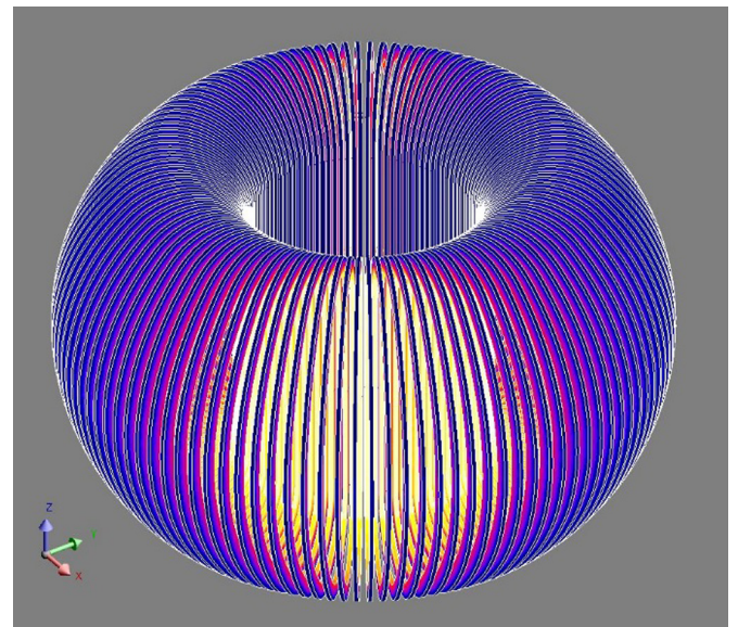
Fig. 10. View of the complete modular toroid, with 112 single pancakes.
