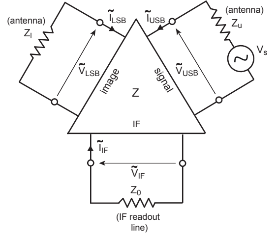
FIG. 7: Equivalent circuit of the Josephson mixer connected to the external impedances Z_u , Z_l and Z_0 .
