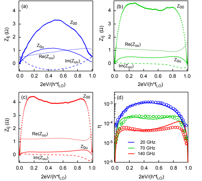
FIG. 8: Main elements of the scattering matrix as a function of normalized voltage calculated at T=58\text{K} for f_{\text{LO}}=20\text{ GHz} (panel a), f_{\text{LO}}=70\text{ GHz} (panel b) and f_{\text{LO}}=140\text{ GHz} (panel c). d) Comparison between experimental (dots) and theoretical (full lines) conversion efficiency \eta_C calculated for the three LO frequencies.
