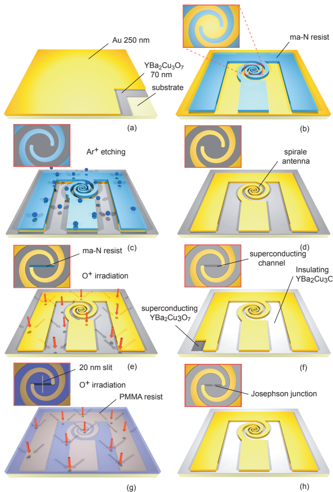
FIG. 1: Illustration of the fabrication process steps: (a) 70-nm thick \text{YBa}_2\text{Cu}_3\text{O}_7 film grown on sapphire covered by an in situ 250-nm gold layer; (b) spirale antenna in the CPW transmission line defined in an ma-N negative e-beam resist; (c) 500-eV \text{Ar}^+ ion-beam-etching; (d) gold antenna in the CPW transmission line on \text{YBa}_2\text{Cu}_3\text{O}_7 ; (e) high-dose 70-keV oxygen ion irradiation to create insulating regions in exposed \text{YBa}_2\text{Cu}_3\text{O}_7 . A 2\text{-}\mu\text{m} wide channel in the center of the antenna is protected by a ma-N resist mask; (f) patterned superconducting and insulating \text{YBa}_2\text{Cu}_3\text{O}_7 regions; (g) low-dose 110 keV oxygen ion irradiation of the Josephson junction patterned as 20-nm-wide slits in PMMA photoresist; and (h) device after resist cleaning.
