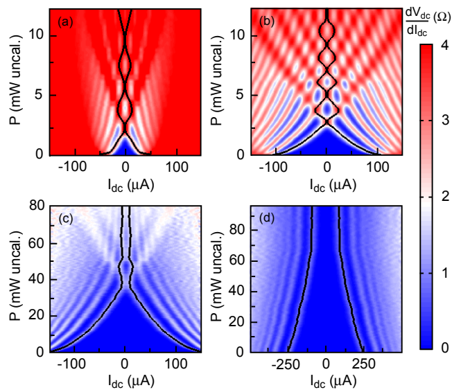
FIG. 5: Differential resistance of junction (color scale) under a 20-GHz LO signal as a function of bias current and RF power for different temperatures : (a) T=56K; (b) T=53K; (c) T=42K; (d) T=35K. The critical current (n=0 step) as a function of RF power is shown in full back line. Complete oscillations of the current height of the Shapiro steps can be seen only in the Josephson regime T'_c < T < T_J (panels (a)–(c)). In the flux flow regime, the critical current is never reduced to zero.
