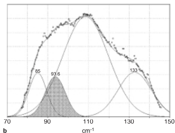
Figure 10 Decomposition procedure to extract XRD (a) and FIR (b) indexes of PCI (gray) for the contact sample at surface.
