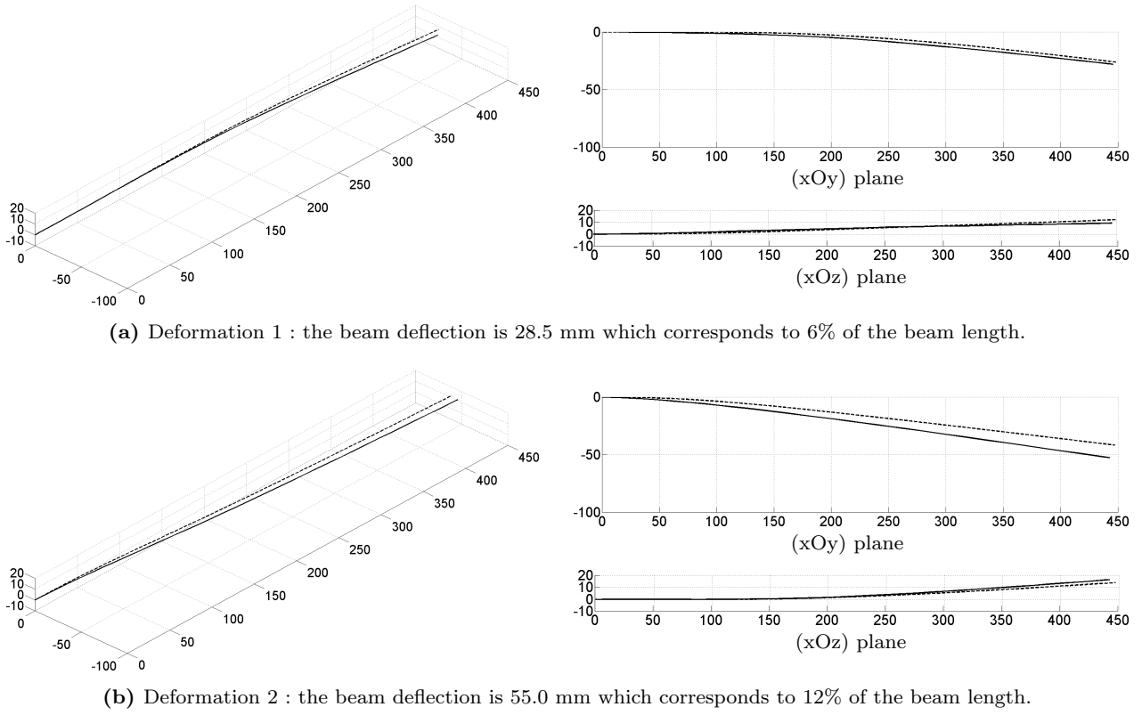
Fig. 9 Original shape (plain) and reconstructed shape (dotted) of a 3D deformed beam. Loads are located at 250 mm and 400 mm directed towards the (Oz) and (Oy) axis. Units are in millimeters.
