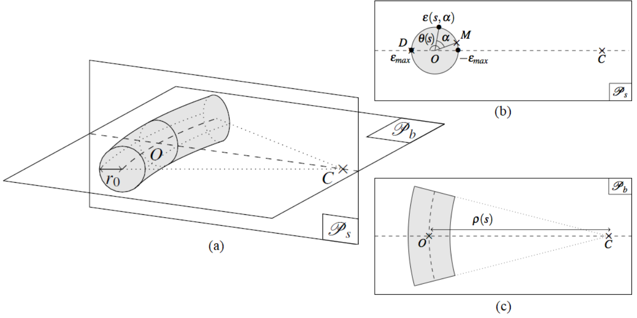
Fig. 1 Deformation of a beam element
