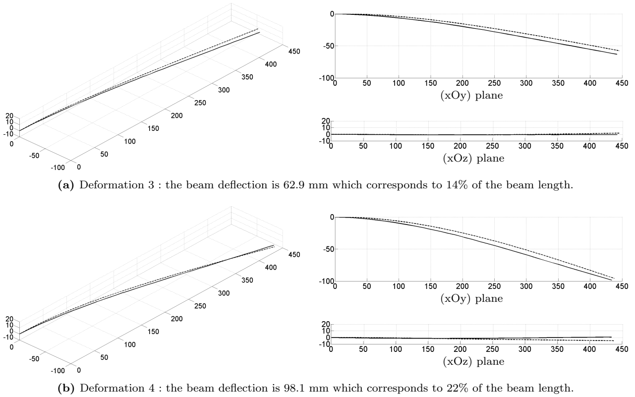
Fig. 10 Original shape (plain) and reconstructed shape (dotted) of a 2D deformed beam. Loads are located at 400 mm directed towards the (Oy) axis. Units are in millimeters.
