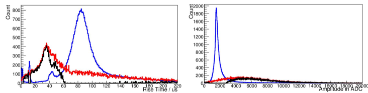
Figure 9: Left panel is the rise time distribution of the signal; right panel is the amplitude spectra (Blue: background; red with \alpha source; black: pure source with background subtracted).
