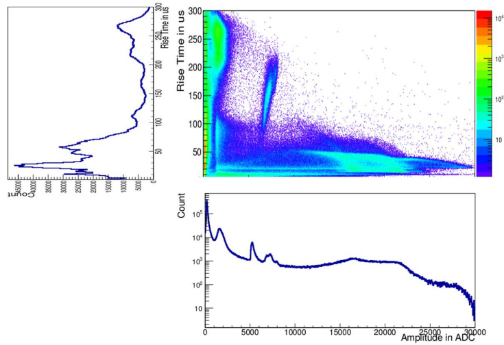
Figure 5: The 2D graph of pulse rise time and amplitude with the \alpha source.
