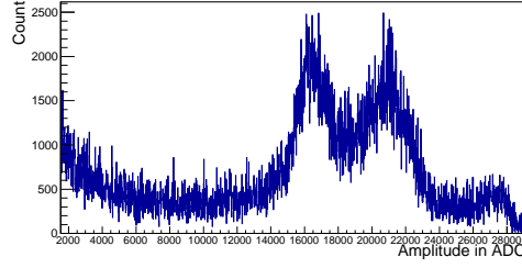
Figure 6: Amplitude spectrum with rise time cut [25, 30] \mu\text{s} for \alpha .
