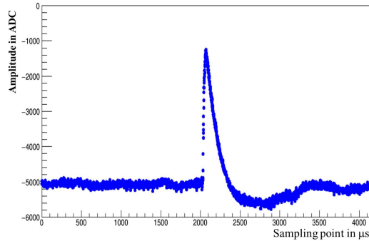
Figure 3: Sampled waveform: X axis is the sampling time in \mu\text{s} and Y axis is the pulse amplitude in ADC.
