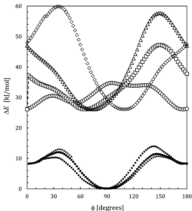
Fig. 6 Energy profiles of D (hollow markers) and T (solid markers) cells containing one CO 2 molecule, as a function of the angle \theta . Several \phi orientations are represented for each cell, passing in front of different steric interaction regions, as illustrated in Fig. 5. Markers are as follows: for D cell, circles, \phi_1 ; squares, \phi_2 ; diamonds, \phi_3 ; and triangles, \phi_5 ; for T cell, circles, \phi_1 ; squares, \phi_2 ; and triangles, \phi_3 .
