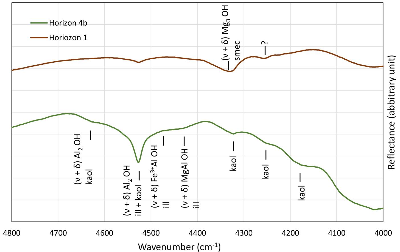
Fig 8. Near infrared reflectance on fine clay material of horizon 1 and 4. \nu and \delta denote stretching and bending, respectively.
