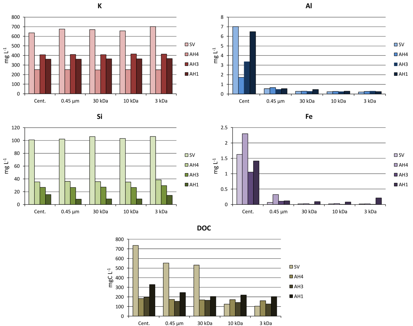
Fig 10. Si, K, Fe, Al and DOC contents in solutions after centrifugation and subsequent filtration at 0.45 μm, 30 kDa, 10 kDa and 3 kDa. SV denotes Salina Verde and AH are auger holes shown along cross section in Fig 4.
