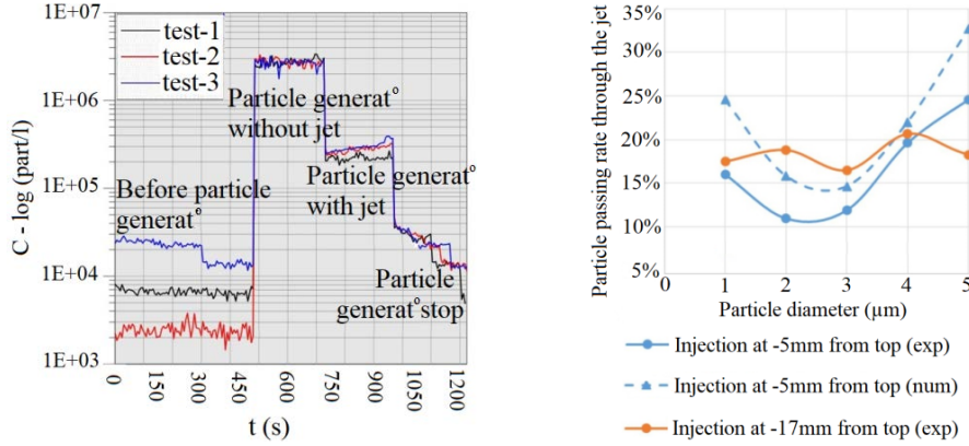
Fig. 7. Time evolution of the particle concentration (left). Evolution of the passing rate of the particles through the jet with respect to the particle diameter (right).
