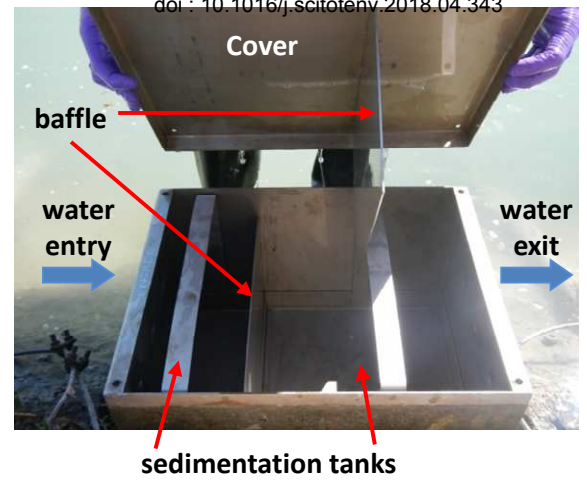
Figure 2: Scheme and picture of the particle trap (PT) used to collect SPM; A=250 mm, B=400 mm, C=300 mm.
