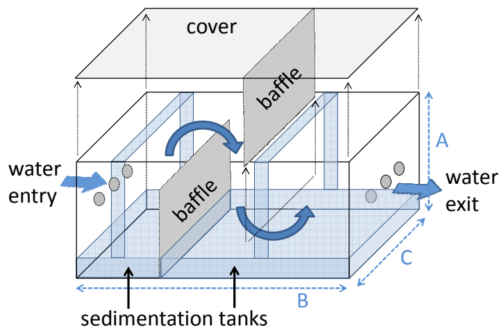
Figure 2: Scheme and picture of the particle trap (PT) used to collect SPM; A=250 mm, B=400 mm, C=300 mm.
