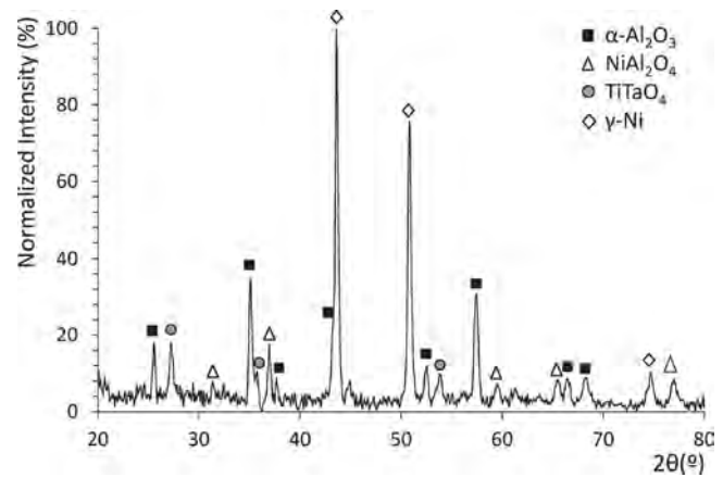
Fig. 7. X-ray diffraction pattern of the Pt + Al \gamma - \gamma' coating after 12,810 cycles at 1100 °C (PA-1 sample).
