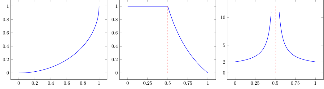
Figure 3: Plot of \varphi_{0.5}(u) with u on the x-axis (vertical slope at u = 1 ). Plots of \varphi_q(1) and \mathbb{E}(\text{Ev}_{\text{lab}}(\langle (M_q)\underline{Q}^l, \varepsilon \rangle)_l \mid \langle (M_q)\underline{Q}, \varepsilon \rangle \downarrow \underline{Q}) with q on the x-axis. See Example 7.
