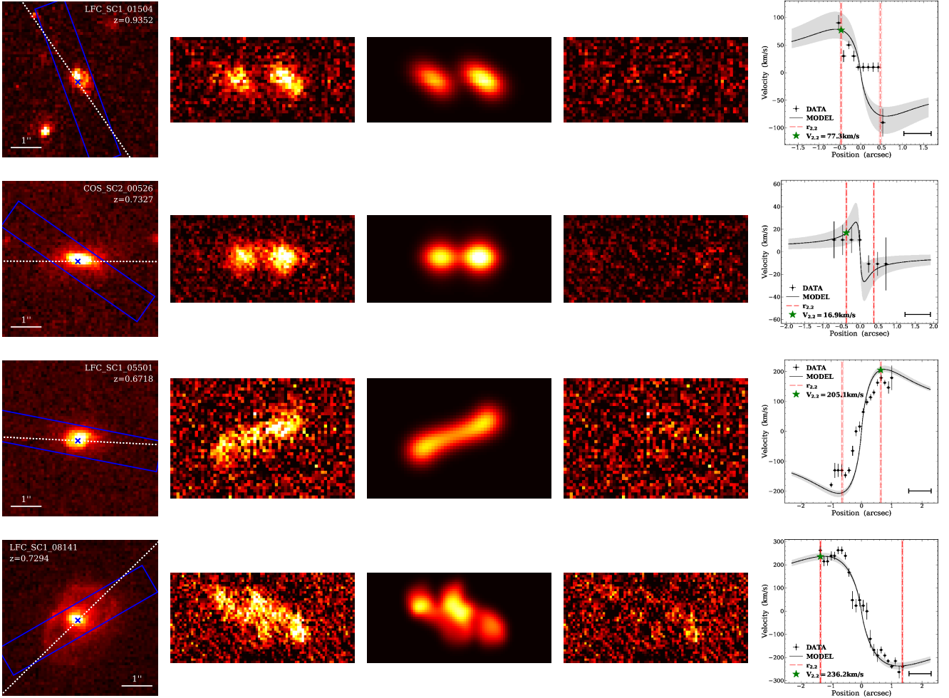
Figure 2. Examples of the kinematic modeling for four galaxies with [\text{O II}] and \text{H}\beta emission. These galaxies have stellar masses typical of the four stellar mass bins used in the analysis in Sec. 4.3, which span the entire range from low (top) to high (bottom) M_* . Each row: From left to right: HST / ACS F814W postage stamp ( 5'' \times 5'' ) with superimposed in blue the DEIMOS slit and in white the orientation of the galaxy PA; continuum-subtracted 2D spectrum centered at the emission line; best-fit kinematic model; residual image between the 2D spectrum and the best-fit model on the same intensity scale as the 2D spectrum; high-resolution rotation curve model (black line), corrected for the inclination, with 1\sigma uncertainty (shaded area), compared to the observed rotation curve (black points). The red dashed and dotted lines indicate the radius r_{2,2} (see Sec. 4.1) and its uncertainty, respectively. The horizontal black bar on the bottom right corner represents the DEIMOS spatial PSF.
