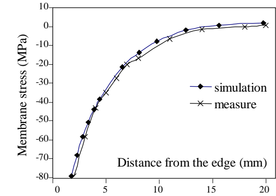
Figure 6. Comparisons between predicted and measured membrane stresses close to the edge (the measures started from the chamfer)
