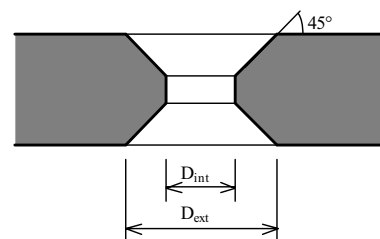
Figure 1. Chamfered holes
