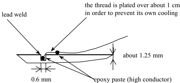
Figure 5. Description of the thermocouples
