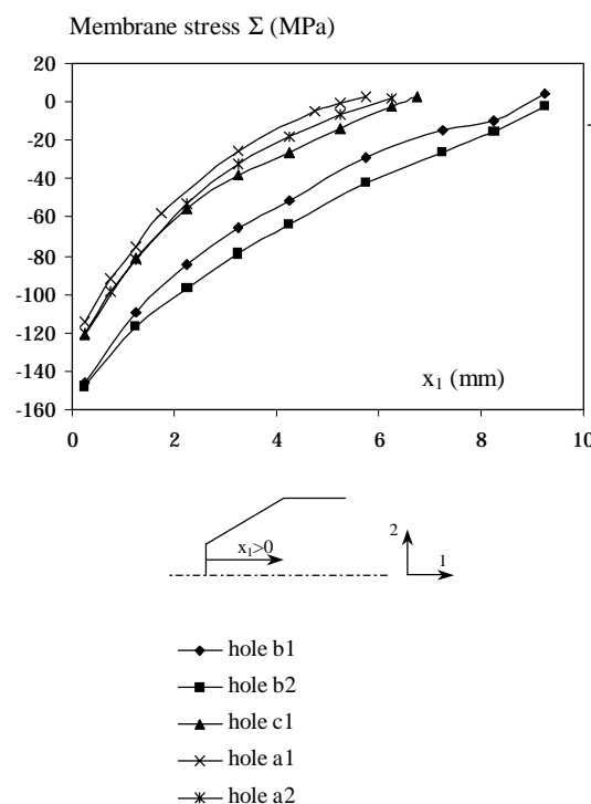
Figure 9. Predicted membrane stress
