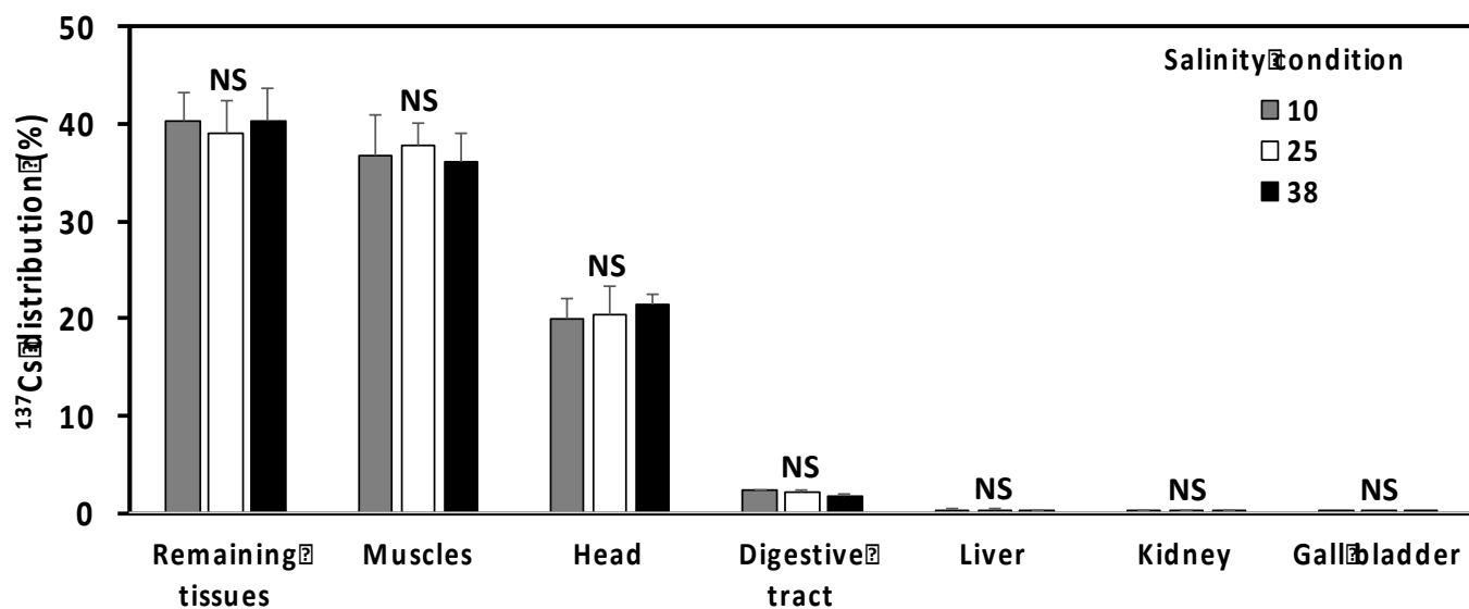
Figure 3. Distribution (%) of ^{137}\text{Cs} in the tissues of juvenile turbot acclimated to three salinity conditions (10, 25 and 38), single-fed with ^{137}\text{Cs} -radiolabelled pellets and then maintained for 21d in non-contaminated seawater at the given salinity. Values are means \pm SD (n=4).
