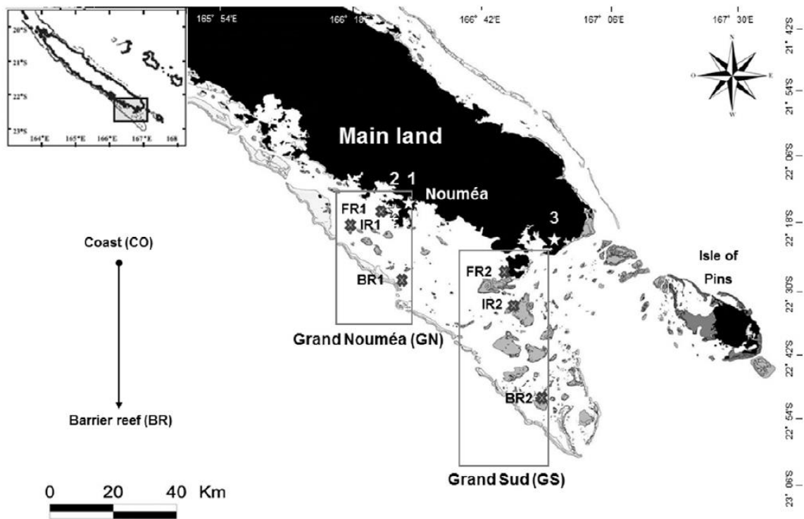
Figure 1. Study site locations in the southwest lagoon of New Caledonia, SW Pacific Ocean. Six sites distributed on a coast-barrier reef gradient (fringing reef FR, intermediate reef IR and barrier reef BR) were sampled in two different areas referred to as Grand Nouméa (GN, area 1) and Grand Sud (GS, area 2). Stars indicate zones of human activities: the industrial area of Ducos (1), the Nickel factory SLN (2), and the Nickel factory Vale-NC (3). The emerged land is indicated in black; grey areas represent coral reefs; the dark grey line represents the slope of the barrier reef.
