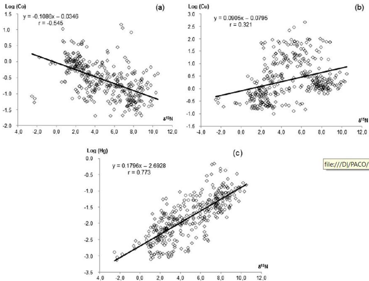
Figure 3. Relation between trophic level ( \delta^{15}\text{N} ) and trace element concentrations (logarithm base ten) along food webs, all trophic compartments pooled. The elements (a) Co, (b) Cu and (c) Hg are presented as examples, all demonstrating significant linear regressions ( p < 0.001 ).
