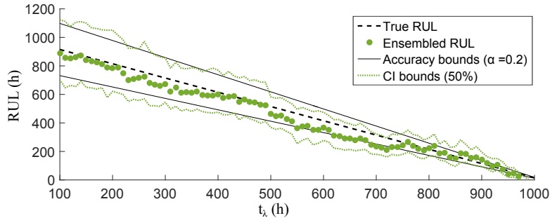
Figure 16: Aggregated RUL predictions with uncertainty for trajectory N o 40 with accuracy and confidence interval (CI) bounds.
