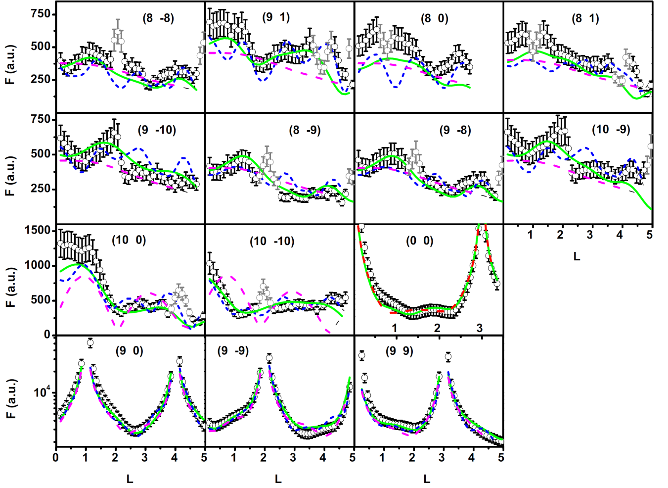
FIG. 4. (Color online) SXR dataset taken in UHV after deposition of 0.2 ML Pt on graphene/Ir(111): Black and grey circles with error bars are measured structure factors whereas grey data points contain scattering contributions from a small amount of larger sintered clusters and are excluded from fitting. There are four different fit curves: i) long dashed (magenta) lines - fit with flat sp^2 hybridized graphene ii) short dashed (blue) lines - comparison with DFT model iii) long dashed (red) line - fit with final model with only 10 % occupation in the second cluster layer (only in specular (0,0) rod - third row and column) iv) solid (green) line - fit with final model including a corrugated graphene model with sp^3 hybridized area below cluster. The first two rows contain cluster lattice rods without any contribution of the Ir(111) bulk. The third row contains rods, where the cluster lattice signal gets a strong coherent contribution from the graphene layer. The bottom row displays crystal truncation rods and the interference between the Ir bulk crystal and the Pt cluster lattice contains information on the position of the cluster in the unit cell.
