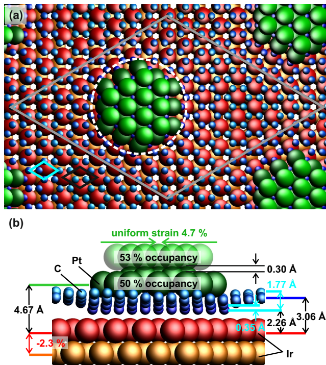
FIG. 5. (Color online) Model used to fit SXR data: (a) Top view of moiré unit cell (grey). 10x10 carbon unit cells (blue) fit commensurately on top of 9x9 Ir(111) unit cells (black). A two layer high cluster sits on top of the carbon layer where the carbon rings are above fcc sites in respect to the Ir support. The edge atoms of the cluster (bright green) are allowed to vary their height with respect to the rest of the layer. The white circle marks the determined diameter of GISAXS measurements. (b) Side view of the SXR model with fitted parameters. Cluster (green) on top of the graphene layer (blue) and two layers of the Ir(111) substrate (red, orange).
