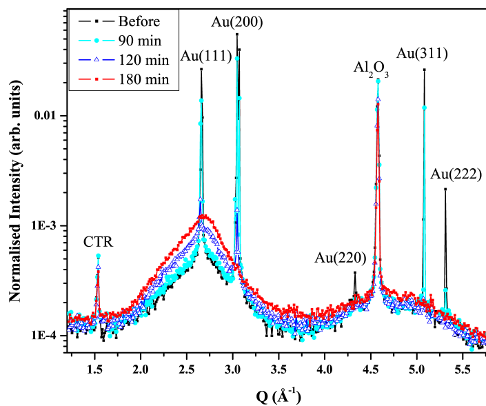
Fig. 8. GIXD radial scan, along the [\bar{2}11] azimuth ( \alpha_i = 0.2^\circ ), showing the melt of 4 nm Au during 0.6 sccm \text{SiH}_4 exposure: Au melt achieved after 180 min of gas exposure.
