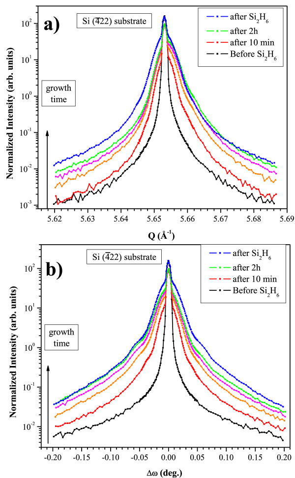
Fig. 14. GIXD ( \alpha_i = 0.16^\circ ), during growth at 790 K: 5 ML Au, exposure to 0.6 sccm \text{Si}_2\text{H}_6 for 120 minutes: a) radial scan along the [\bar{2}11] direction; b) \omega rocking curves around the \text{Si}(\bar{4}22) Bragg peak
