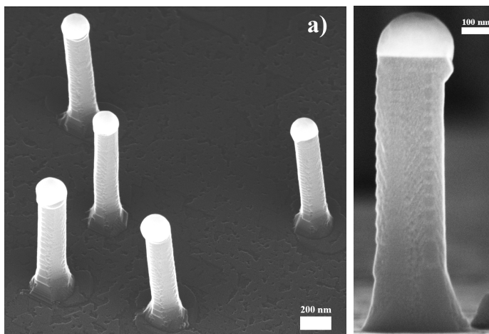
Fig. 15. SEM after growth at 790 K: 5 ML Au, exposure to 0.6 sccm \text{Si}_2\text{H}_6 for 120 minutes. Sample inclined of a) 45^\circ and b) 80^\circ
