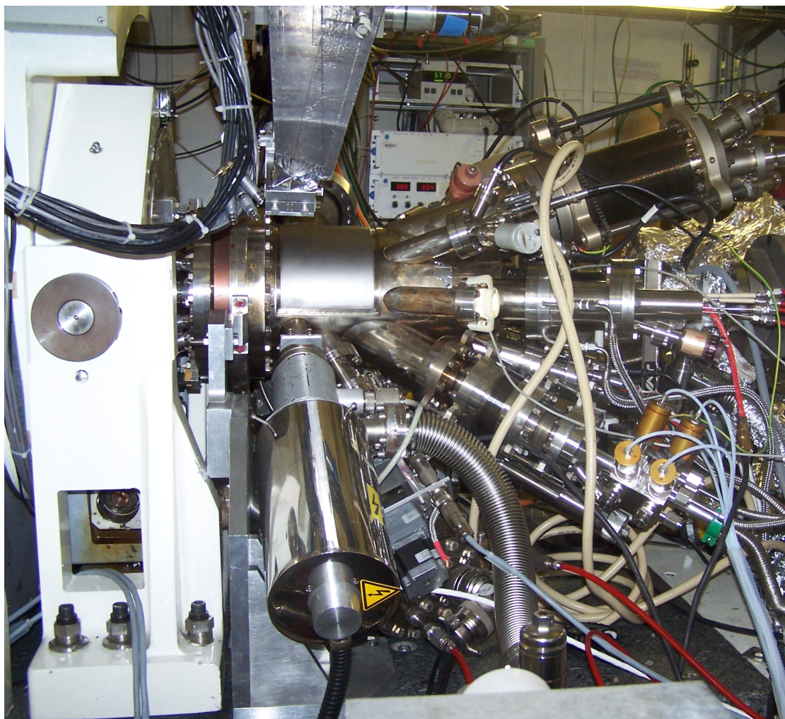
Fig. 2. Photograph of the core of the INS set-up viewed from the direction opposite to the incoming X-ray beam (detector side). A small part of the heavy-duty diffractometer carrying the UHV chamber is visible on the left (white and steel parts), while most of the picture is occupied by the UHV deposition chamber. The large exit Be window is clearly visible in the center of the picture. The slit/detector system for GIXD measurements is toward the top. The CVD gas injector is visible on the bottom right corner below a Si MBE source. Other sources (such as a Omicron EFM4) can be distinguished. The RHEED gun is visible at the bottom, and the AES set-up on the top right (into a large bellows). The large ion pump is integrated into the diffractometer below the chamber, and the turbomolecular pumps are on the other side.
