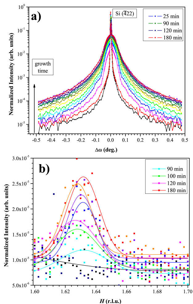
Fig. 16. GIXD ( \alpha_i = 0.08^\circ ), during growth at 770 K: 1.75 ML Au, exposure to 0.15 sccm \text{Si}_2\text{H}_6 for 180 minutes: a) \omega rocking curves around the \text{Si}(422) Bragg peak; b) radial scan along the [\bar{1}11] direction
