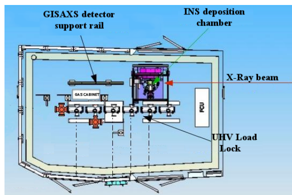
Fig. 5. Technical drawing of the INS experimental hutch BM32 (EH3): the different equipments are shown and indicated into the figure.
