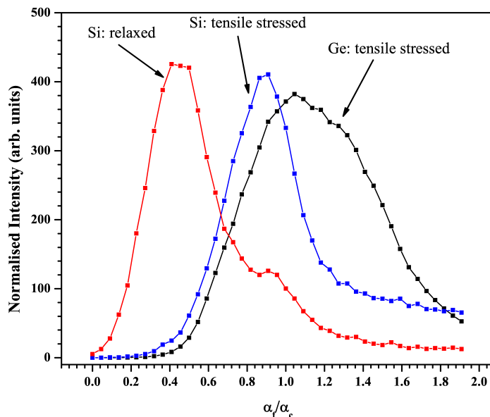
Fig. 12. \alpha_f/\alpha_c ( \alpha_c = 0.22^\circ for Ge) curves collected after growth at 740 K. The peak integration was performed using another ROI having the size of 20 (H) \times 20 (V) pixels, corresponding to a detector acceptance of 1.7 mrad in both directions centred at the pixel position of the Ge substrate Yoneda peak \alpha_c . The x-ray diffraction patterns as function of the exit angle are collected in a way that the diffracted signal is hitting always the same detector pixel position.
