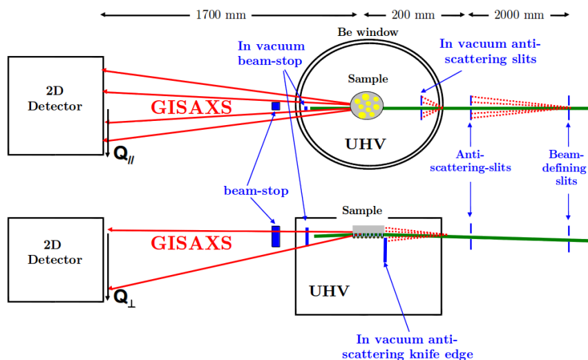
Fig. 4. Sketch of the slit system for GISAXS measurements on the INS/BM32 set-up. The incident beam is depicted by a green line coming from right. Slits, anti-scattering slits, knife edge and beam-stop are pictured in blue. The small angle x-ray scattering is symbolised by red arrows.
