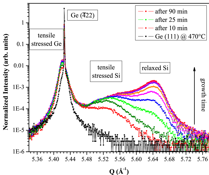
Fig. 11. GIXD ( \alpha_i = 0.1^\circ ), during growth at 740 K: exposure to 0.3 sccm of \text{Si}_2\text{H}_6 for 90 minutes. The intensity was integrated in a region of interest (ROI) having the size of 232 (H) \times 18 (V) pixels, corresponding to a detector acceptance of 20 (H) \times 1.5 (V) \text{mrad}^2
