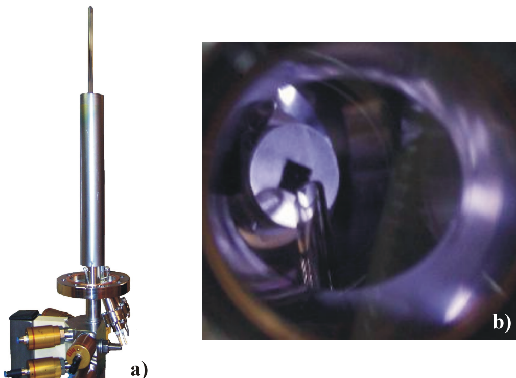
Fig. 7. a) Picture of the Riber CVD gas injector with its quartz tube; b) View inside the chamber through a viewport showing the end of the quartz tube approaching the sample.
