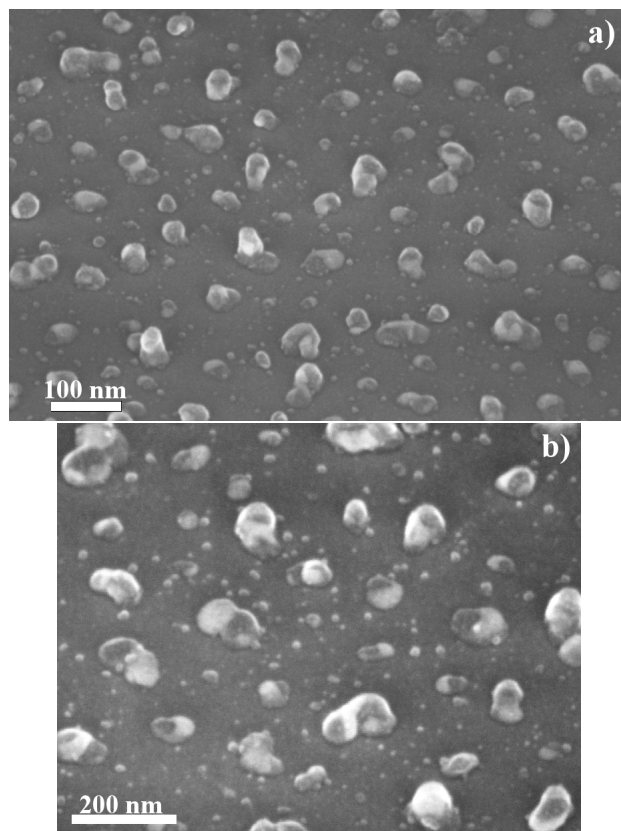
Fig. 13. SEM micrographs of UHV-CVD grown Si nanostructures on Ge(111).
