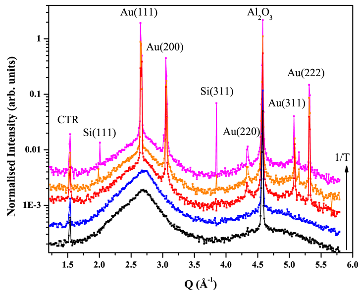
Fig. 9. GIXD radial scan, along the [\bar{2}11] azimuth ( \alpha_i = 0.2^\circ ), showing the solidification of 4 nm after exposure to \text{SiH}_4 : Au solidification achieved with a \Delta T \cong 50 \text{ K} (intensities scaled for clarity).
