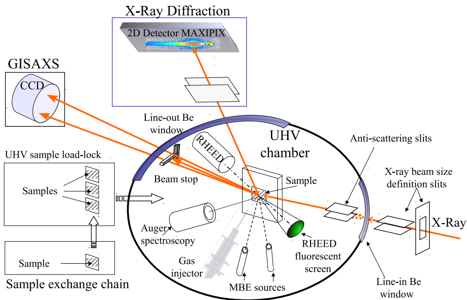
Fig. 1. Principle of the INS/BM32 UHV chamber coupled to the diffractometer for in situ GISAXS and GIXD measurements. The last vertical anti-scattering slits of the beamline are placed inside the UHV chamber to suppress unwanted x-ray scattering from the entrance Be window. A knife edge can be approached close to the sample to further reduce the background in the horizontal direction. A beam stop is placed inside the chamber just before the exit Be window to block the main beam before it hits the Be window, which would otherwise generate unwanted background scattering. An additional beam stop can also be added outside to remove residual background. RHEED and AES conclude the sample analysis possibilities. The chamber can be equipped with up to 8 PVD/MBE sources. All apparatus are oriented toward the center of rotation of the diffractometer allowing x-ray measurements during nanostructure formation. Sample introduction is performed through a load-lock and a storage/introduction UHV chamber.
