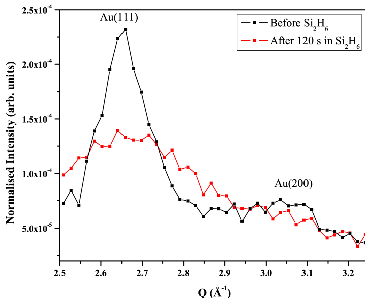
Fig. 10. GIXD \delta scans ( \alpha_i = 0.16^\circ ), showing the melting of 16 Å polycrystalline Au after 120 s exposure to \text{Si}_2\text{H}_6 .
