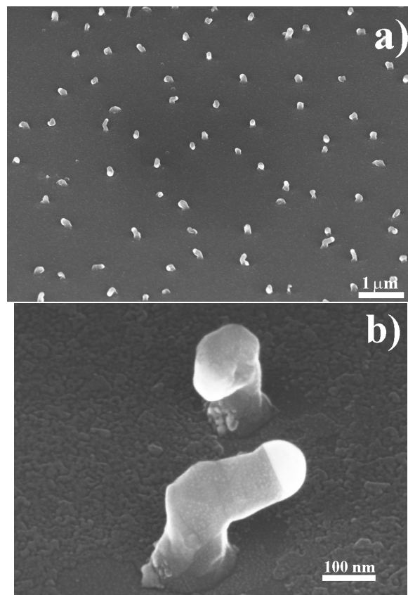
Fig. 17. SEM (sample inclined of 45^\circ ) after growth at 770 K: 1.75 ML Au, exposure to 0.15 sccm \text{Si}_2\text{H}_6 for 180 minutes.
