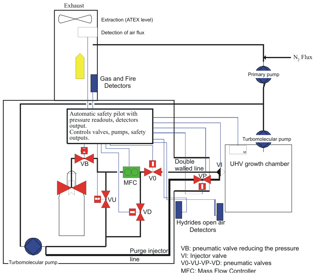
Fig. 6. Schematic diagram of the gas injection system for CVD growth. Only one gas injection line is represented; three are available.
