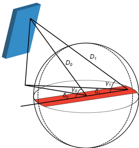
Figure 9 Graphic representation of the divergence problem. Each pixel in the two-dimensional detector detects photons scattered from a different part of the sample at different scattering angles, both in plane and out of plane.
