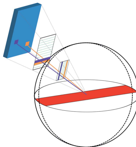
Figure 10 The use of two one-dimensional slits positioned perpendicular to each other to solve the divergence problem and the border issue.
