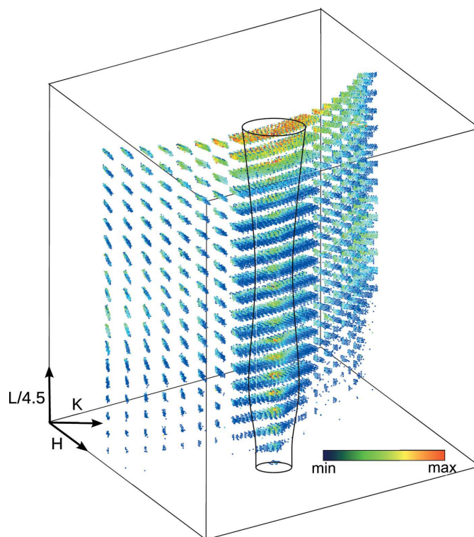
Figure 11 Reconstruction of a surface rod in reciprocal space [ (\frac{2}{3}, 0, l) rod of a CsO layer adsorbed on Pt(111)]. The reciprocal intensity map was reconstructed from rocking scans taken at different l . For this particular rod we used dense sampling in proximity to the rod (depicted as a deformed cylinder) and fewer images were taken in the background region.
