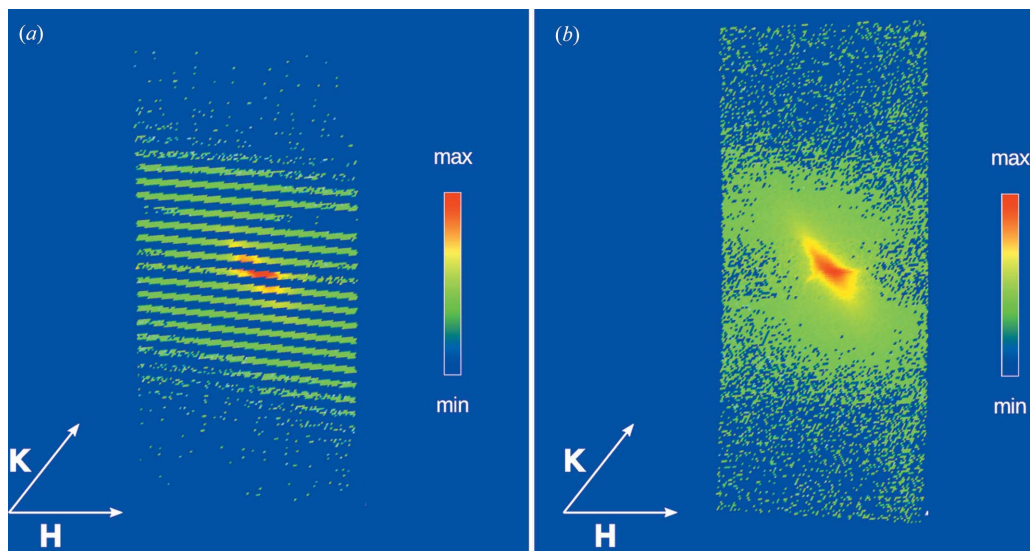
Figure 12 The projected intensity for a (1, 0, l) CTR with l = 0.45 (a) and l = 2.65 (b) [clean Pt(111), log scale].
