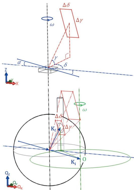
Figure 1 (Top) Graphic representation of the angle convention in real space (in the reference system of the diffractometer). The incident beam is confined in the XZ plane, while the sample surface is parallel to the XY plane. (Bottom) Graphic representation of the angle convention in reciprocal space. For elastic scattering we have |\mathbf{K}_i| = |\mathbf{K}_f| . The point \mathbf{O} denotes the reciprocal space origin. A homogeneous crystal truncation rod is added (black cylinder); the intersection with the Ewald sphere is illustrated as a deformed ellipse; the sample surface plane is shown as a grey circle, while the green circle depicts the reciprocal plane \mathbf{Q}_{\perp} = 0 . Also shown is the projected detector acceptance onto the Ewald sphere, given by K_f \Delta \gamma and K_f \Delta \delta .
