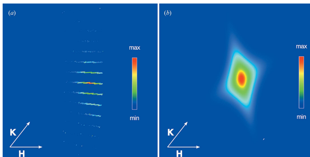
Figure 16 (a) The in-plane projection of the rocking curve [(\frac{2}{3}, 0, l) surface rod of a CsO layer on Pt(111) measured at l = 0.45 ]. (b) Lorentzian fit of the in-plane projection. Intensity is in log scale.
