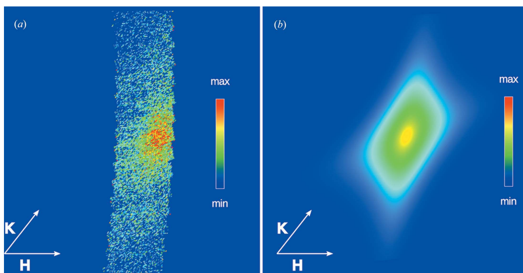
Figure 15 (a) The in-plane projection of the rocking curve [(\frac{2}{3}, 0, l) surface rod of a CsO layer on Pt(111) measured at l = 2.40 ]. (b) Lorentzian fit of the in-plane projection. Intensity is in log scale.
