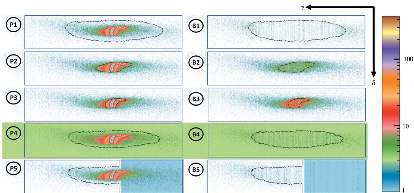
Figure 4 A demonstration of the robustness of the peak search algorithm. The intensity is illustrated by false color levels and is in logarithmic scale. In each case a peak search is performed inside the rectangular-shaped RoI, followed by a background estimation within the same region. The resulting peak is indicated by the black contour. On the left: the peak found on the original, unmodified image. On the right: the background estimated within the peak contour to be subtracted pixel by pixel before the final integration.
