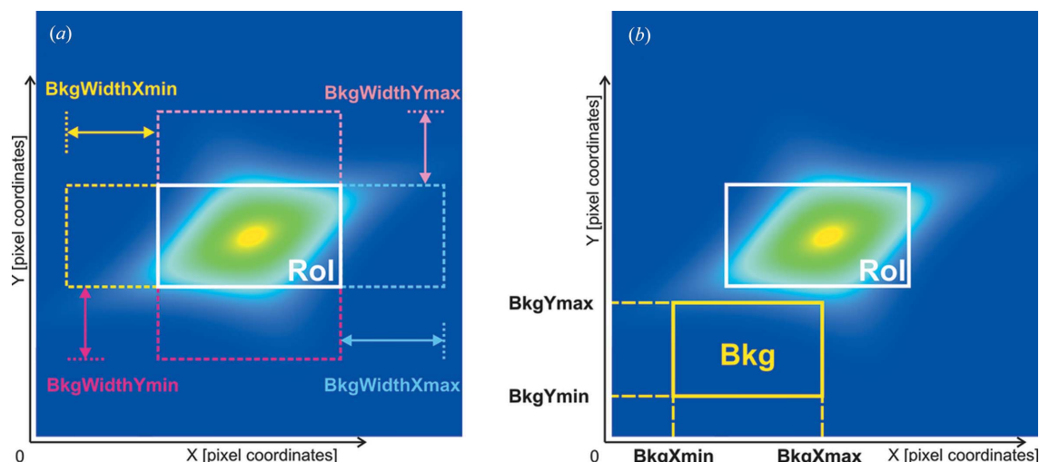
Figure 3 Different ways of selecting the background: (a) rectangles adjacent to each RoI edge; (b) rectangular area outside the RoI.
