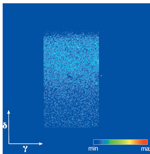
Figure 14 Image with the maximum intensity in the rocking curve [(\frac{2}{5}, 0, l) surface rod of a CsO layer on Pt(111) measured at l = 2.40 ]. Intensity is in log scale.
