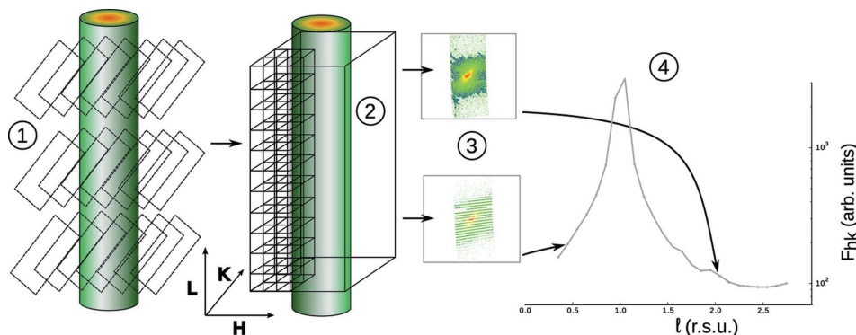
Figure 13 Summary of the integration in reciprocal space: rocking scans at various l values are taken (1), a reciprocal space map is constructed (2), l_{\text{const}} (in-plane) projections are integrated or interpolated and then integrated (3), and |F_{hkl}| is determined (4).
