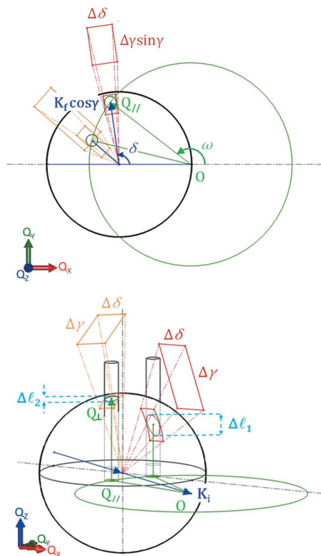
Figure 2 (Top) Top view of two stationary measurements of the same rod at different l values. The in-plane projection of the finite acceptance of the detector is proportional to \sin \gamma and thus is smaller for lower l values (red) than for higher l values (orange). The measurement is only valid if the projected rectangle is large enough to contain the rod cross section (small green circle). (Bottom) Perspective view of the same measurements. Integration should only be carried out if the intensity distribution is approximately uniform along l within the intercepted range \Delta l , which itself is proportional to \cos \gamma . The condition is thus generally easier to fulfill at higher l values (orange) than for lower l values (red).
