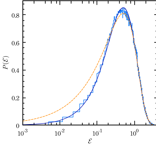
Fig. 2 Histogram of the normalized field component amplitude from experimental data, compared with the prediction (2) (continuous line) and the corresponding probability distribution of P_{\epsilon}(\epsilon) where the value d = 0.89 was used. Weibull best fit (dashed curve).
