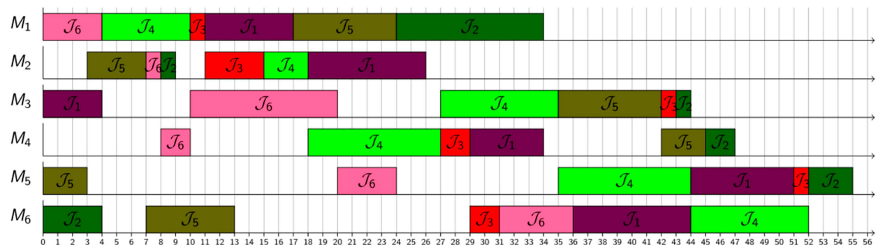
Figure 6. An alternative schedule obtained by swapping a dispatching decision at machine 2 from Figure 5.
