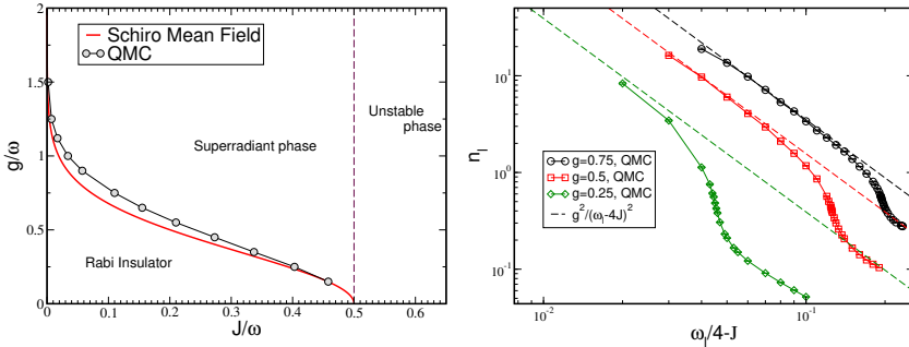
Fig. 2 (left) The QMC phase diagram of the Rabi Hubbard model, compared with mean field results. We observe two phases: an incoherent Rabi insulator and a coherent superradiant phase. There is also a region where the system is unstable for J > \omega_1/2 . (right) Density of photons in the system, as a function of -J . As J approaches the unstable region ( J > \omega_1/4 in this case), the density of photons diverges. As n_l becomes large, it reaches a mean field regime where n_l \simeq g^2 / (\omega_1 - 4J)^2 . See [14] for details.
