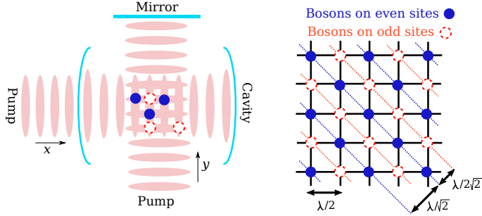
Fig. 3 (left) In the experiment [17], a 2D gas of cold atoms is subjected to two perpendicular modes in a cavity. (right) The two optical modes are coupled if the atoms adopt a chequerboard pattern that provides the right wave planes to couple modes by scattering.
