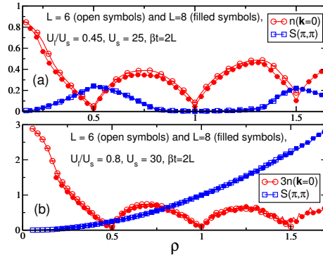
Fig. 5 Varying density, we find different charge density wave, superfluid and supersolid phases. (a) For moderate U_l we find an alternation of phases with ( S(\pi, \pi) \neq 0 ) and without ( S(\pi, \pi) = 0 ) density modulation. (b) For large U_l there is always density modulation.
