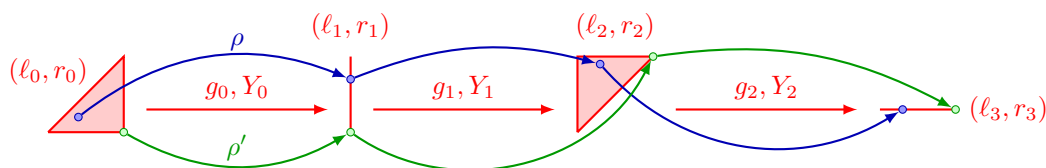
■ Figure 2 A play \rho (in blue), its projected path \pi in the region game (in red), and one of its associated corner plays \rho' (in green).
