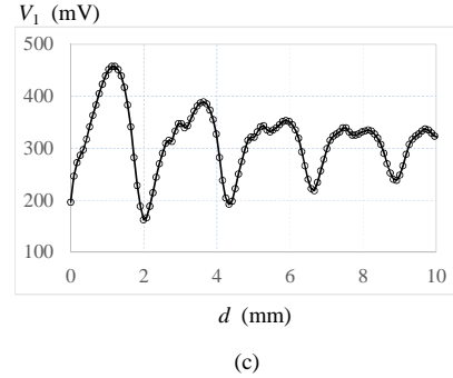
Fig. 5. Free-space distance measurement – F = 60 GHz. (a) and (b) Experimental test bench. (c) Detected voltage V_1 as a function of the stand-off d .
