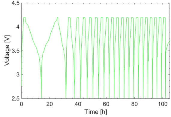
Fig. 3. Voltage response
