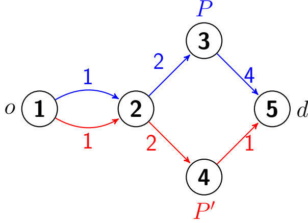
Figure 1: A restricted graph containing two alternative paths for a commodity to be sent from 1 to 5.
