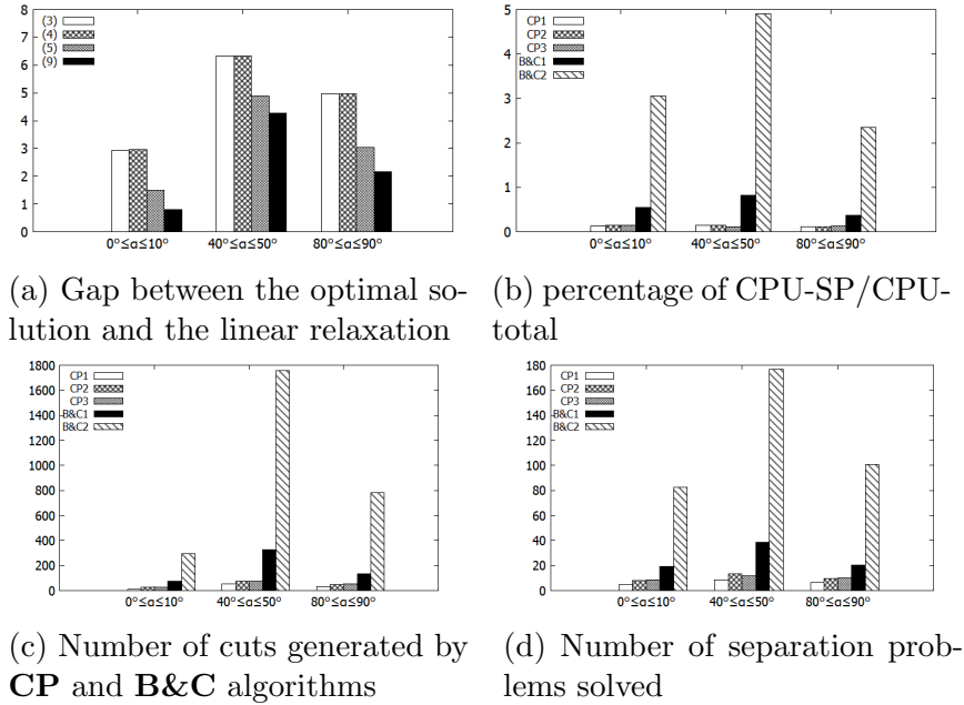
Figure 2: Additional statistics for the algorithms and formulations
