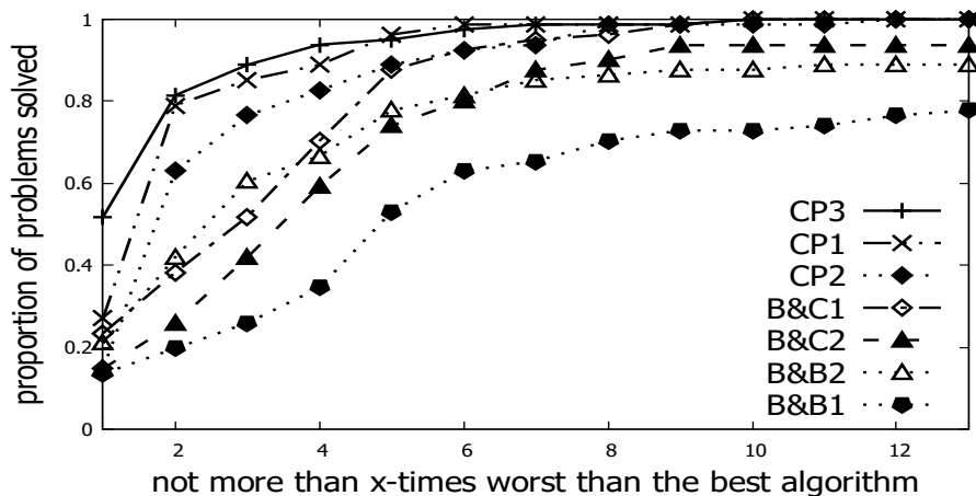
Figure 3: Performance profile comparing the different algorithms for random instances.
