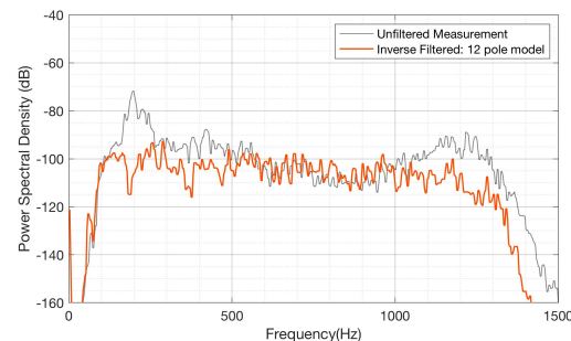
Figure 7: PSD of the inverse filtered result, superimposed on the original PSD estimate. PSD estimates are smoothed with a 3rd order median filter.
