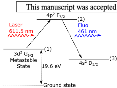
FIG. 1. Basic 1-photon Argon ion LIF scheme. The metastable state is chosen for his long lifetime, and his relative abundance among the ions. The example showed here is the one used in the following experiments.
