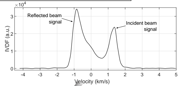
FIG. 4. IVDF showing that the reflected laser beam gives a larger signal intensity than the incident beam. Measured 8 mm away from the ceramic sample.
