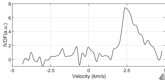
FIG. 6. IVDF measured at 134 mm, with the laser propagating through a 0.8mm hole drilled inside the ceramic sample. P^- vanishes.
