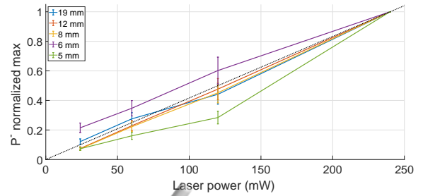
FIG. 7. P^- normalized maximum intensity signal as a function of laser power for the ceramic plate. The intensity at each location is normalized with respect to its value at 240 mW. The black dotted line represents the linear variation, which is the one expected in the non-saturation regime.
