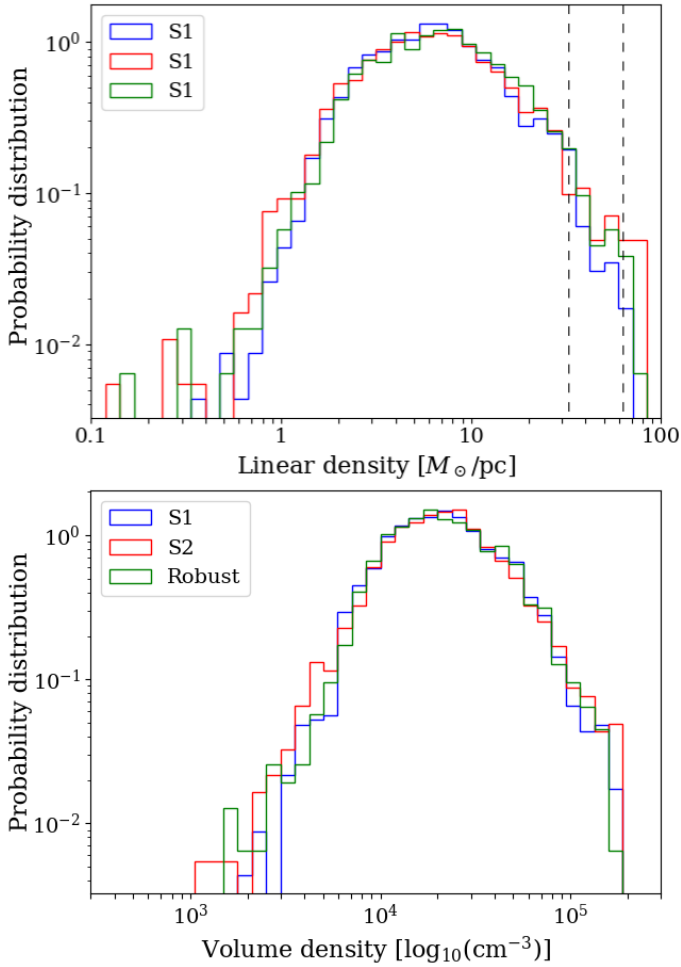
Fig. 11. Top: distribution of the linear density of the filaments. The vertical dashed lines show the most probable critical linear densities corresponding to M_1^{\text{crit}} and M_{\text{1,eff}}^{\text{crit}} . Bottom: distribution of the volume density of the filaments, derived from the linear density and the FWHM of the transverse profiles by assuming a uniform cylindrical geometry. The typical critical volume densities lie beyond the plot, at \gtrsim 3 \times 10^5 \text{ cm}^{-3} .
