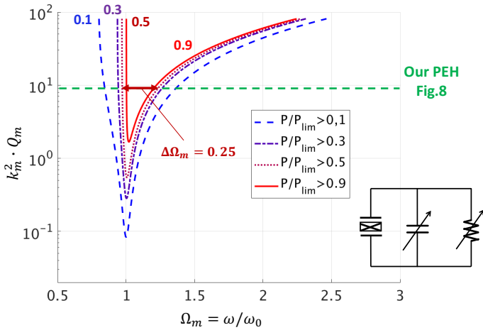
Fig. 4. Normalized analysis of the harvested power with a capacitive tuning interface [9] in the k_m^2 Q_m - \Omega_m plane where Q_m = 20 .
