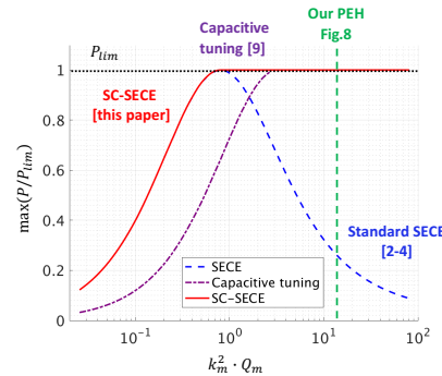
Fig. 6. Maximum harvestable power as a function of k_m^2 Q_m with the standard SECE interface (blue), the capacitive tuning approach (purple), and the proposed SC-SECE (red).
