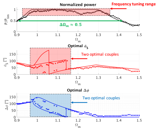
Fig. 9. Experimental (dots) and theoretical (plain lines) maximum harvested power results and optimal (\phi_s, \Delta\phi) .
