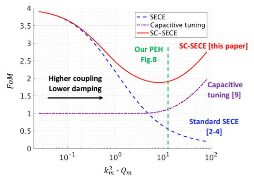
Fig. 7. FoM comparison of the three strategies as a function of k_m^2 Q_m
