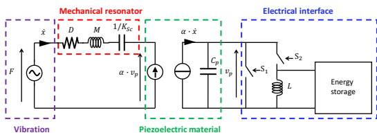
Fig. 1. PEH electrical model and system view of the SC-SECE strategy
