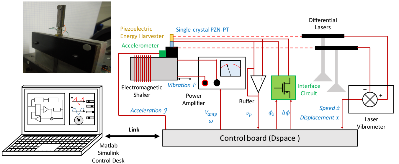
Fig. 8. Experimental setup with automated data collection. The piezoelectric generator is made of 10 \times 5 \times 0.5 \text{ mm}^3 plates of PZN-PT single crystals which have been manufactured by Microfine Company.
