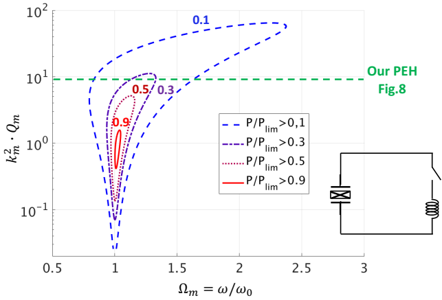
Fig. 3. Normalized analysis of the harvested power with a standard SECE interface [2-4] in the k_m^2 Q_m - \Omega_m plane, where Q_m = 20 .
