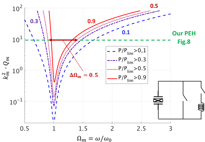
Fig. 5. Normalized analysis of the harvested power thanks to the proposed SC-SECE interface in the k_m^2 Q_m - \Omega_m plane where Q_m = 20 .
