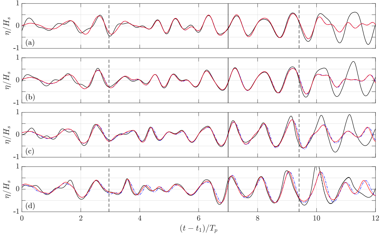
Figure 5: Time series of surface elevation in: (—) laboratory measurements, (— · —) LWT model, and (—) ICWM model, for H_s/\lambda_p = (a) 0.006, (b) 0.018, (c) 0.029 and (d) 0.041. Vertical continuous line corresponds to the reconstruction time t_r , and vertical dashed lines are boundaries of the prediction zone.
