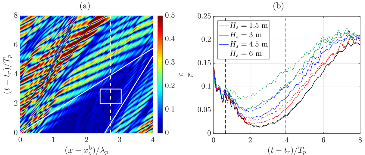
Figure 2: Numerical error of ocean reconstruction: (a) \varepsilon(x, t) using ICWM for one realization with H_s = 3 m; white box marks the spatio-temporal target zone \mathcal{T}(t) , within the prediction zone \mathcal{P}(t) marked by oblique lines; dashed line at x = x_c marks sensor location. (b) \bar{\varepsilon} (averaged over 1,000 realizations) at x = x_c , as a function of time, for different steepness using LWT (---) or ICWM (—); vertical dashed lines mark the prediction zone boundaries.
