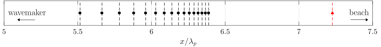
Figure 4: Locations of 16 (out of 20) irregularly spaced wave gauges (●) used in laboratory experiments; (▲) reference wave gauge.
