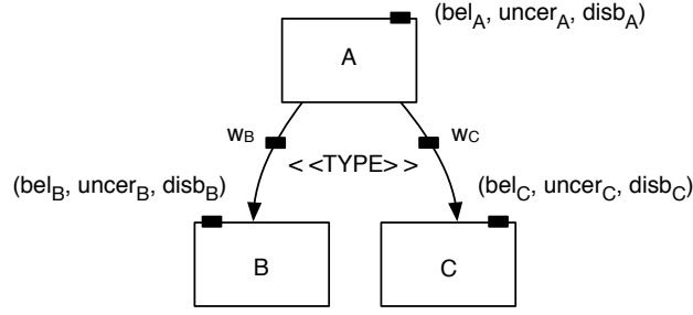
Figure 8: A double-node argument annotated with assessment parameters
