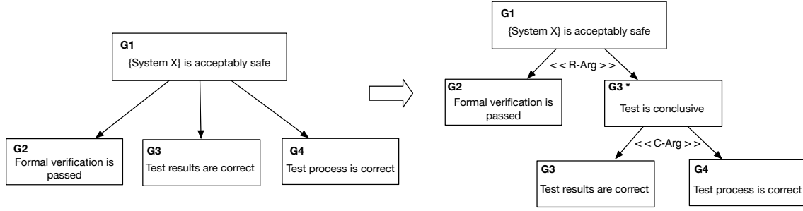
Figure 11: Re-structuring an argument for confidence propagation
