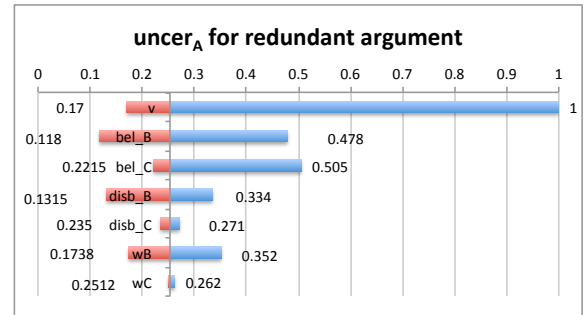
Figure 10: Tornado graphs for two types of double-node arguments
