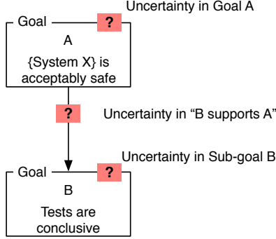
Figure 3: Sources of uncertainties in a simple inference modelled with GSN
