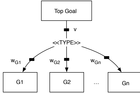
Figure 6: An argument annotated with appropriateness measures
