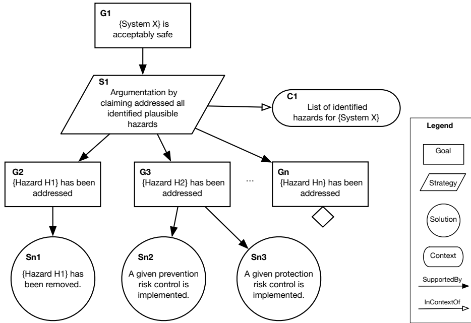
Figure 1: GSN example adapted from the Hazard Avoidance Pattern (Kelly and McDermid, 1997)
