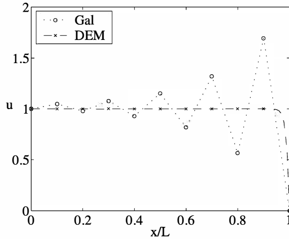
Fig. 23. Homogeneous problem in one dimension, \alpha = 5 .
