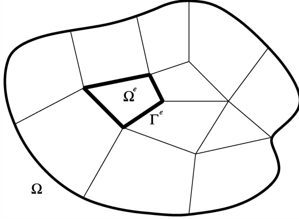
Fig. 1. Domain \Omega partitioned into element domains \Omega^e .
