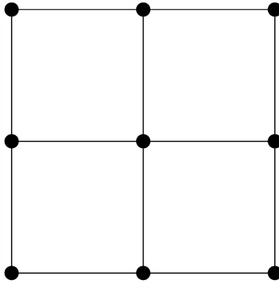
Fig. 14. A nine-node patch.
