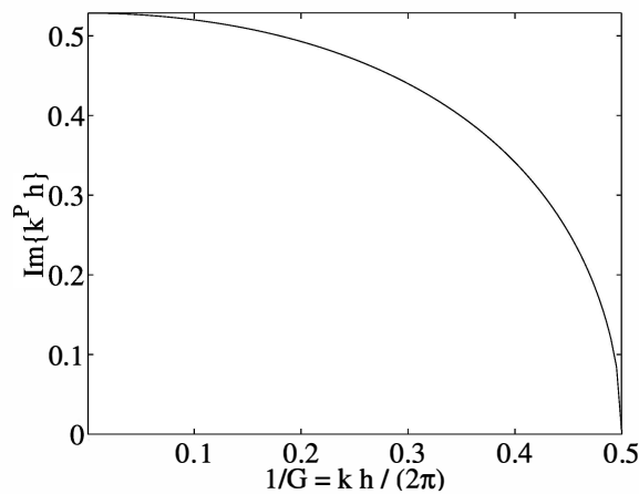
Fig. 2. Damping in polynomial field in one dimension.
