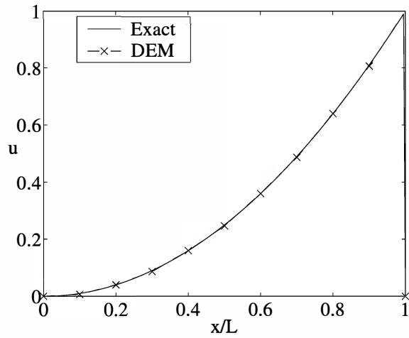
Fig. 26. Inhomogeneous problem in one dimension, \alpha = 10^6 .
