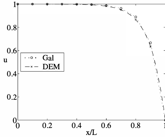
Fig. 22. Homogeneous problem in one dimension, \alpha = 0.5 .
