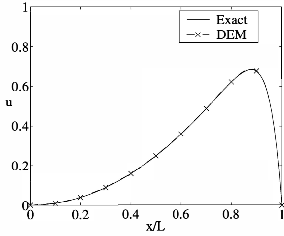
Fig. 24. Inhomogeneous problem in one dimension, \alpha = 1 .
