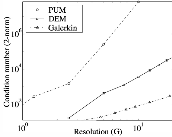
Fig. 21. Condition number at ka = 20 and \theta = 77^\circ .
