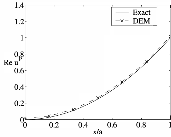
Fig. 6. Particular solution of inhomogeneous problem and u^P in one dimension, ka = 10 , 3.77 points per wavelength.
