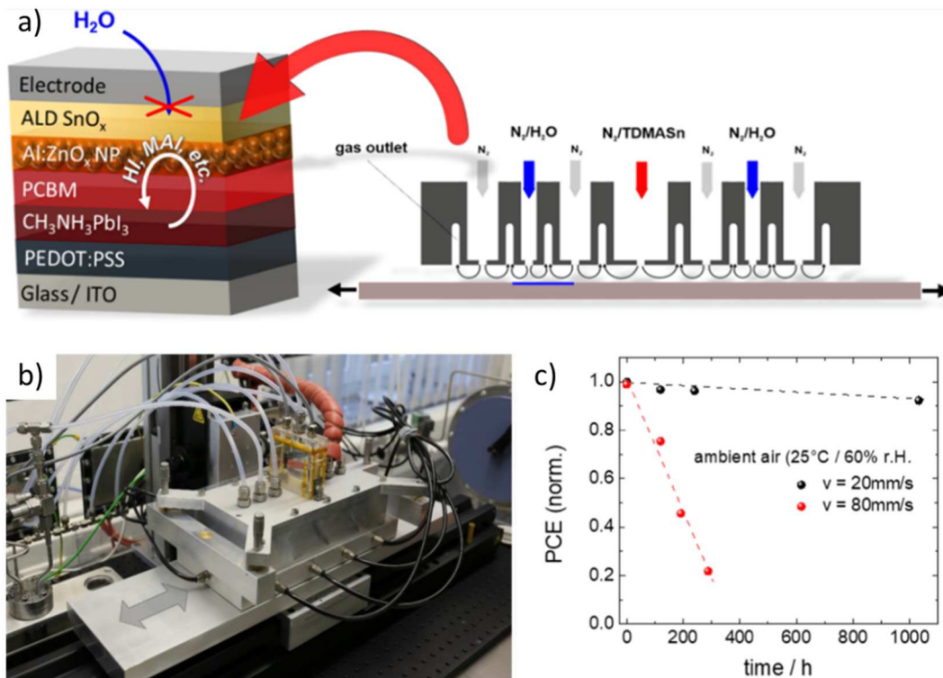
Fig. 17. a) Schematic of the SALD assembly used to deposit a SnO x layer as part of a perovskite solar cell stack; [79] b) Plasma SALD system inside a glove box for the deposition of SnO x layers for solar cells based on hybrid perovskites; c) Normalized photoconversion efficiency (PCE) vs. time of storage in ambient air (25 °C, 60% RH) for solar cells with SALD SnO x layers grown at 20 and 80 mm/s, respectively. (Images courtesy of Prof. T. Riedl);
