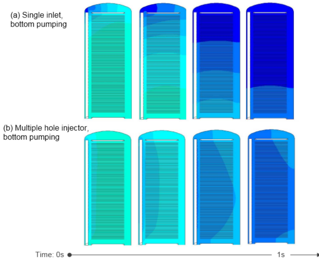
Fig. 2. Contour plots of precursor ( \text{TiCl}_4 ) partial pressure at different times after precursor injection in two similar batch reactors. a) Single inlet reactor. b) Multiple inlet reactor. Reprinted from ref. [24] with permission.
