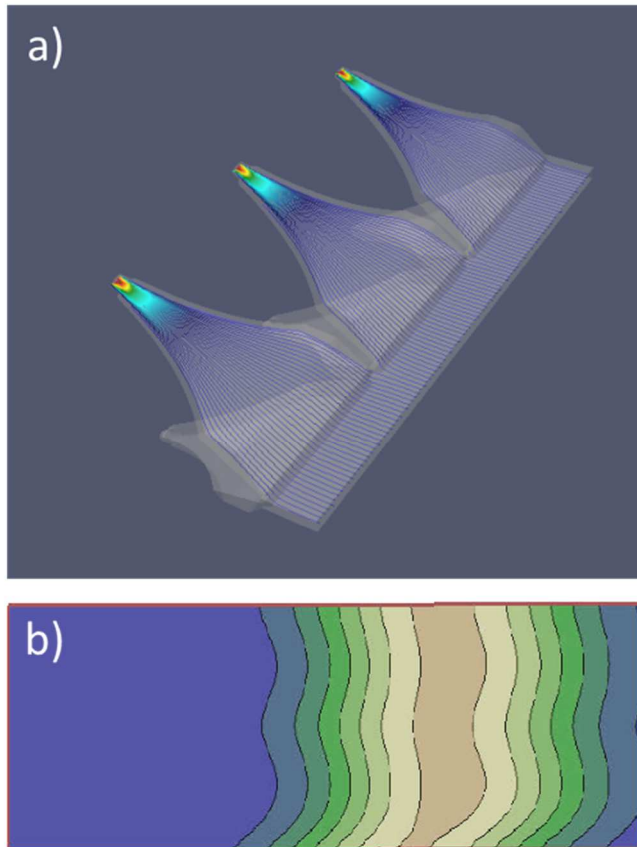
Fig. 7. a) Computational Flow Dynamics Simulation of the gas injectors in the Encapsulix PPW system; b) Precursor concentration isocontours after propagation of the precursor pulse in the reaction space.
