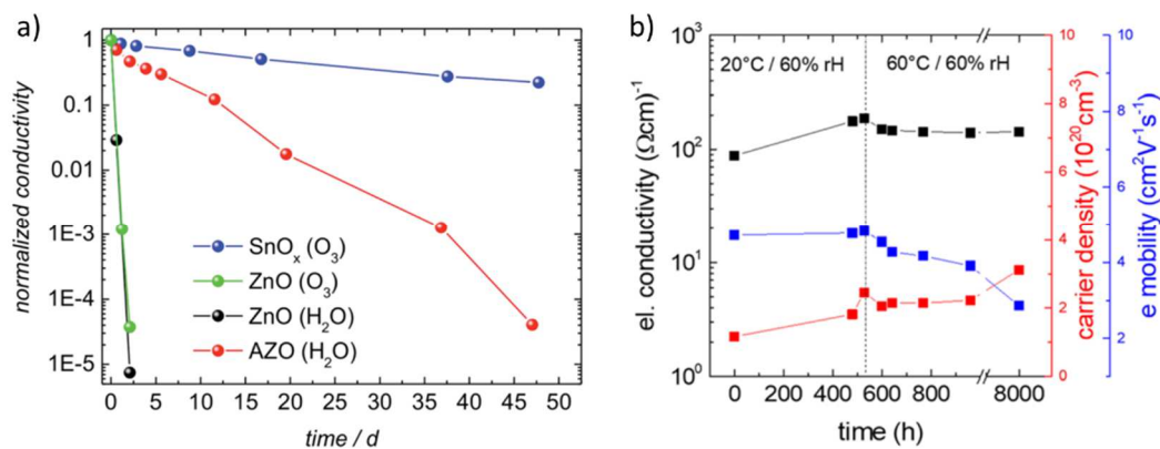
Fig. 20. a) Normalized conductivity upon aging under damp heat conditions (85 °C and 85% RH) of 200 nm thick ZnO, AZO, and \text{SnO}_x films (grown at 150 °C) using \text{O}_3 or \text{H}_2\text{O} as oxidants; b) electrical conductivity, carrier density and electron mobility of \text{SnO}_2 deposited by HT PE-ALD
