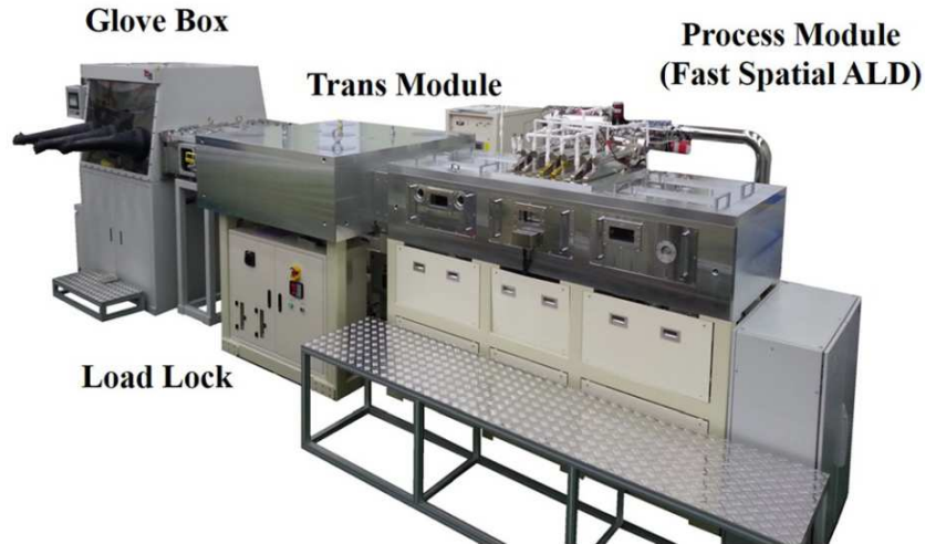
Fig. 15. Photograph of the fast spatial ALD system used by Choi et al. to encapsulate OLED panels.[71]
