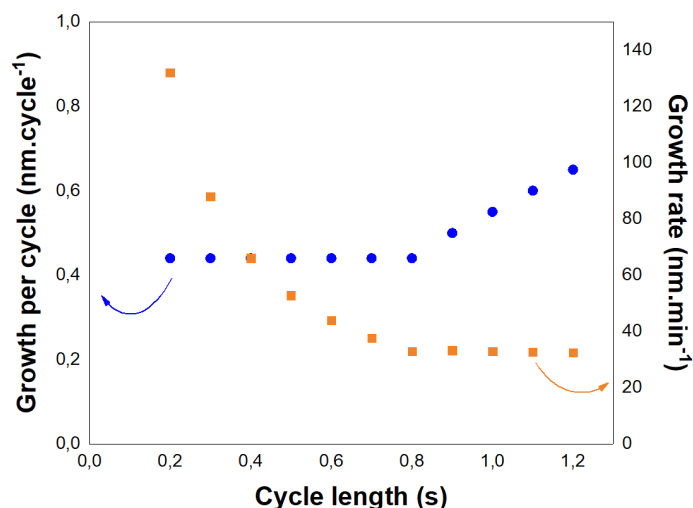
Fig. 12. Evolution of the SiO 2 growth per cycle and growth rate depending on cycle length in FAST deposition mode.
