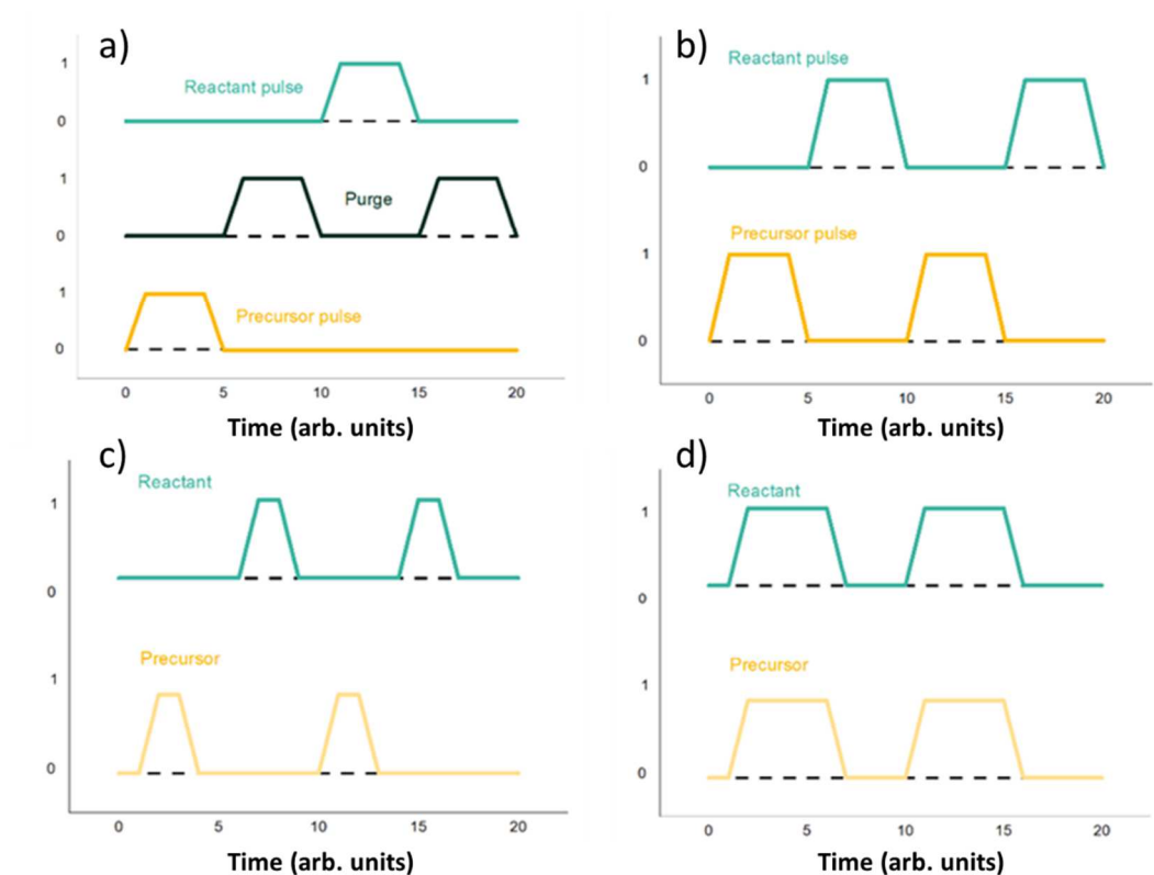
Fig. 9. Sequence of precursor pulses and purges in different operation modes: a) ALD mode, b) FAST mode, c) FAST ALD-like mode, and d) FAST CVD-like mode.
