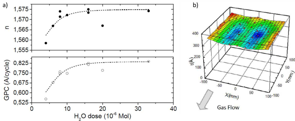
Fig. 18. 25 nm thick \text{Al}_2\text{O}_3 film made in a PPWR Infinity 200 reactor, 3 s/cycle, 90°C. Left: a) optical index ( n ) and GPC vs. the \text{H}_2\text{O} dose; b) non-uniformity of the alumina layer measured on a 200 mm Si wafer
