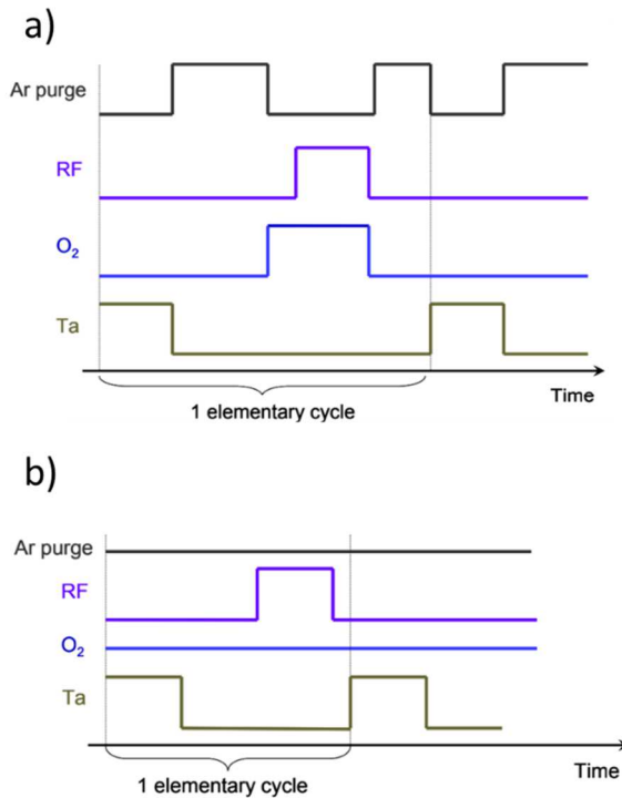
Fig. 11. Comparison of PEALD elementary cycle (a) and engineered-PEALD elementary cycle (b)).
