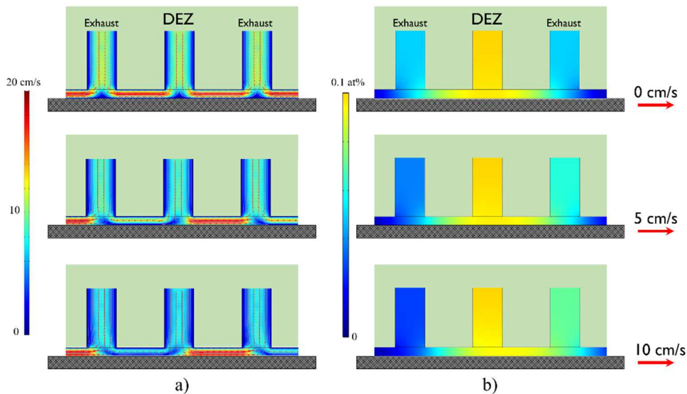
Fig. 13. Spatial distribution of a) Precursor velocity and b) precursor concentration above the substrate for the deposition of ZnO from diethyl zinc (DEZ) with a close-proximity head such as the one in Fig. 2 . Only the cross-section views including a DEZ inlet and two exhaust inlets are shown here. The blue color corresponds to low velocity/precursor concentration, while red or yellow color corresponds to high velocity/precursor concentration. As it can be appreciated, more precursor entrainment takes place as scanning speed increases.
