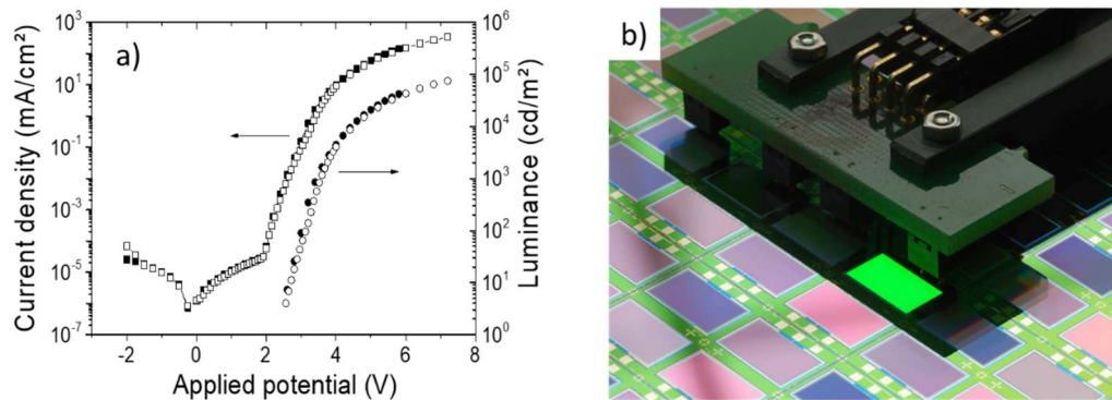
Fig. 19. a) IVL characteristics of a green top-emitting OLED encapsulated with a single 25 nm-thick \text{Al}_2\text{O}_3 barrier layer deposited by HT ALD (3 s/cycle, 90 °C, TMA/ \text{H}_2\text{O} ) in an Infinity 200 tool from Encapsulix - initial time, freshly-made device (filled symbols) and after 22 months in laboratory atmosphere (open symbols); b) picture of the green-emitting OLED surface under 3.2 V forward bias, after 22 months (no dark spots, similar quality as freshly-made device).
