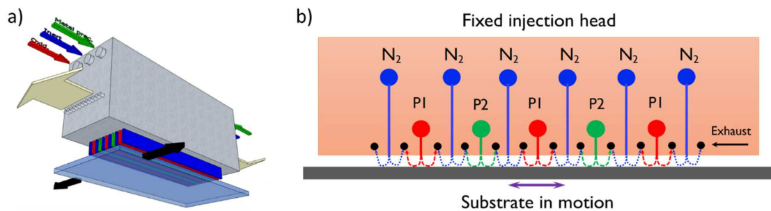
Fig. 3. a) Scheme of a SALD close-proximity head in which the substrate is oscillated below the slots through which the different precursors are continuously injected. B) Side view of the head-substrate gap showing the paths of the different flows that take place for the small gap used, which ensure no precursor crosstalk.
