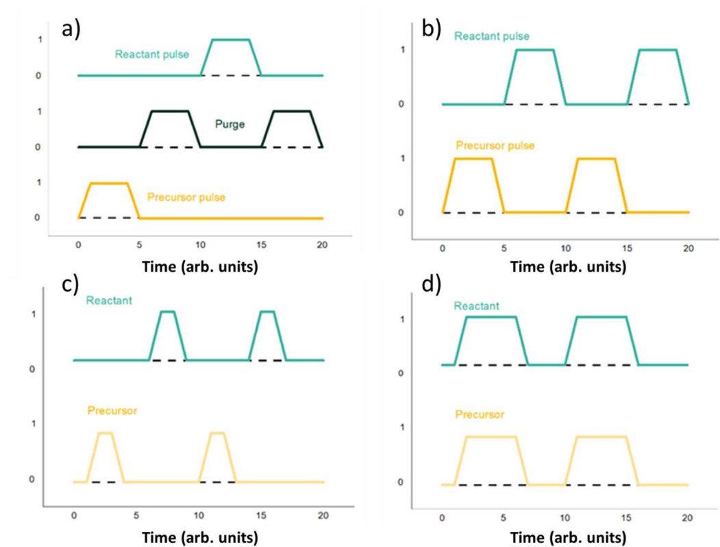
Fig. 9. Sequence of precursor pulses and purges in different operation modes: a) ALD mode, b) FAST mode, c) FAST ALD-like mode, and d) FAST CVD-like mode.
