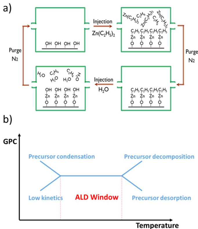
Fig. 1. a) Scheme of the Atomic Layer Deposition (ALD) process for the deposition of ZnO, showing the alternative steps: a first precursor (DEZ, diethylzinc) is injected and a purge occurs followed by the injection of the second precursor (water) and so on. b) Scheme of the typical Growth per Cycle (GPC) as a function of temperature in ALD.
