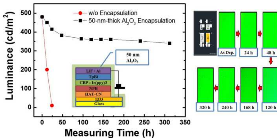
Fig.16. Emission lifetime evaluation of Al 2 O 3 encapsulation on an OLED panel.
