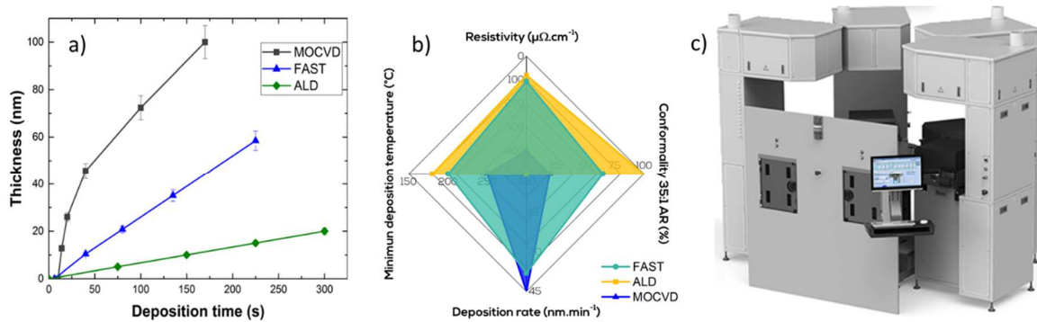
Fig. 10. a) Variation of TiN deposition rate from TDEAT and \text{NH}_3 by ALD, MOCVD, and FAST techniques. b) Comparison of ALD, CVD and FAST deposition techniques for the deposition of TiN using the same precursors and temperature. c) FAST reactor cluster from KOBUS used to perform the deposition of TiN in the three different modes.
