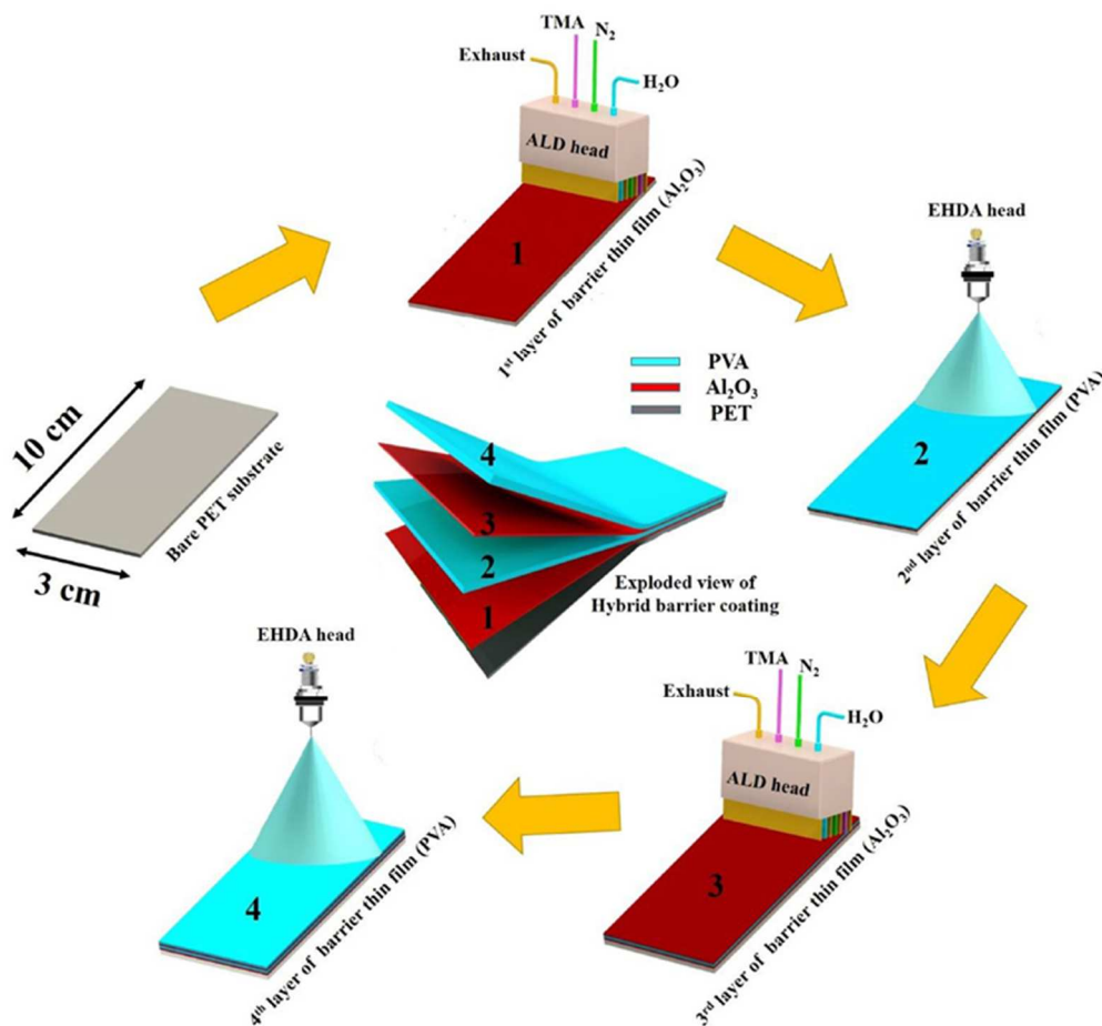
Fig. 22. Flow process diagram of hybrid multilayer barrier coating containing bare PET substrate. [70]
