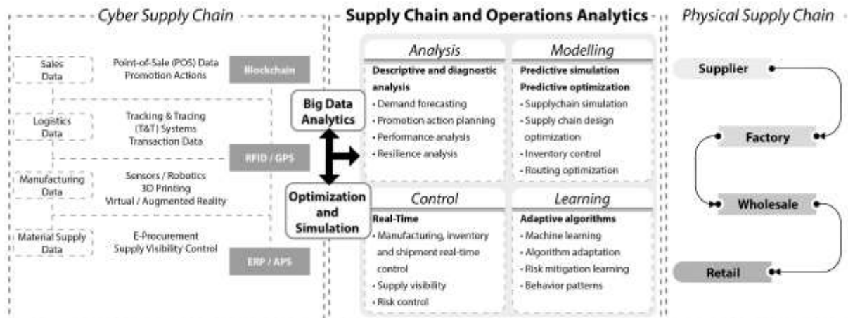
Fig. 4. Digital SC framework
