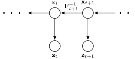
Fig 5: Inverted arrows for the SSM with no observations
